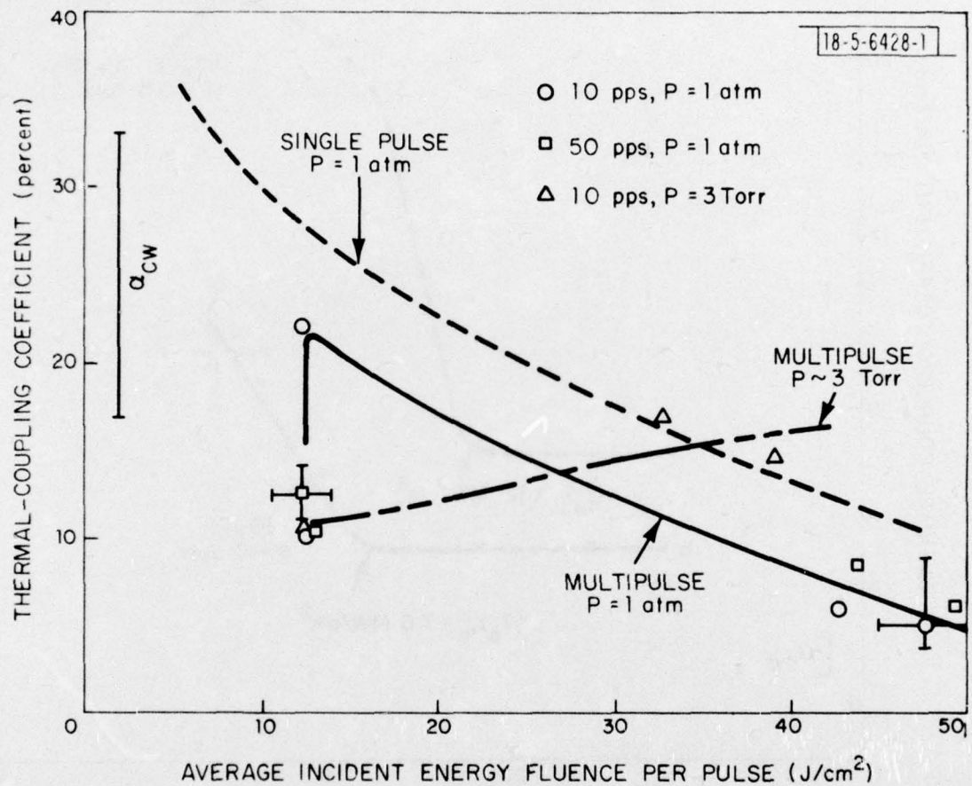
Fig. 8. Thermal coupling coefficient for titanium (6Al-4V). Multipulse ambient atmosphere results (connected by the solid curve for viewing convenience) were measured with a Mach 0.4 air flow transverse to the target surface. The dashed curve represents the single-pulse results of Marcus. 4,5 Low-pressure multipulse results are also shown and connected by the broken curve for viewing purposes.
