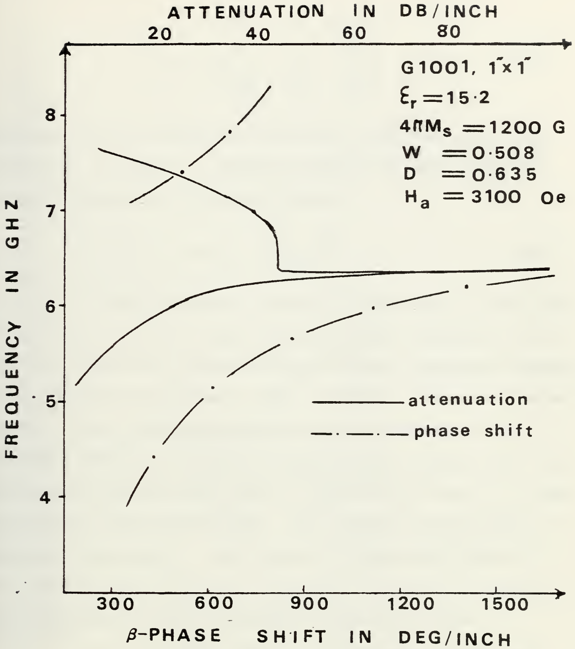
Figure 2-24A. Propagation Constant of Transverse Magnetized Microstrip Transmission Line.
