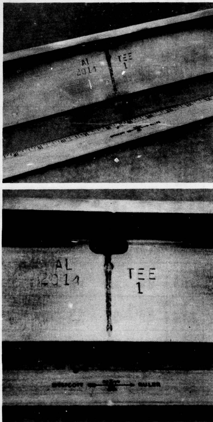
Figure 54 SSEB Butt Weld Made on 0.300-inch-Thick 2014-T651 Aluminum Alloy Tee Shape
