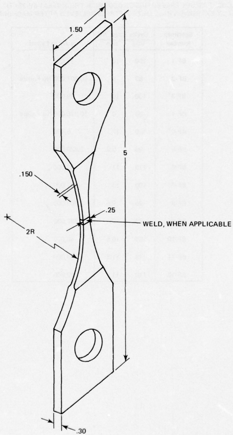
Figure 79 Fatigue Weld Test Specimen (45MPS 240)
