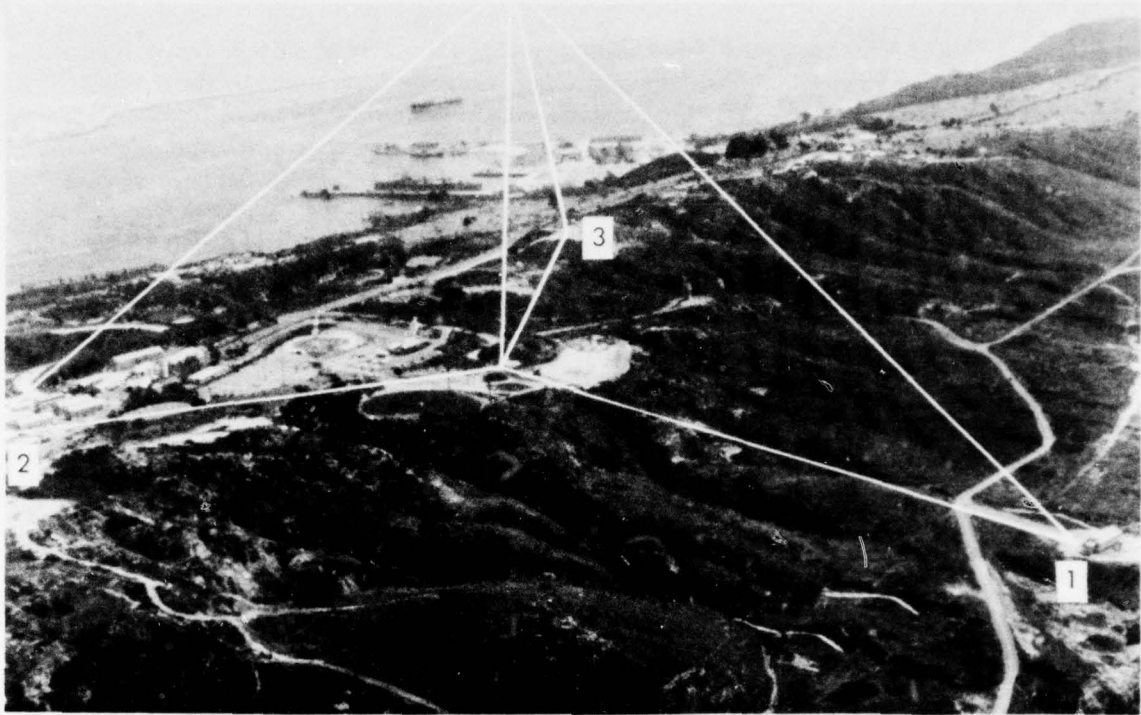
Figure 3. Geometrical configuration of the XONICS acoustic echosounder and wind-sensor system at NELC.
