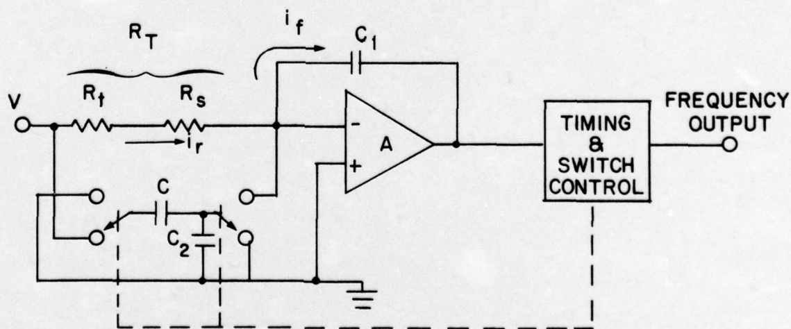
Figure 1 V/F Converter
