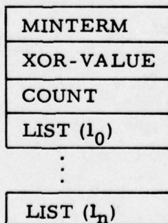
Figure C-1. Pictorial Representation of a MINTERM Item.
