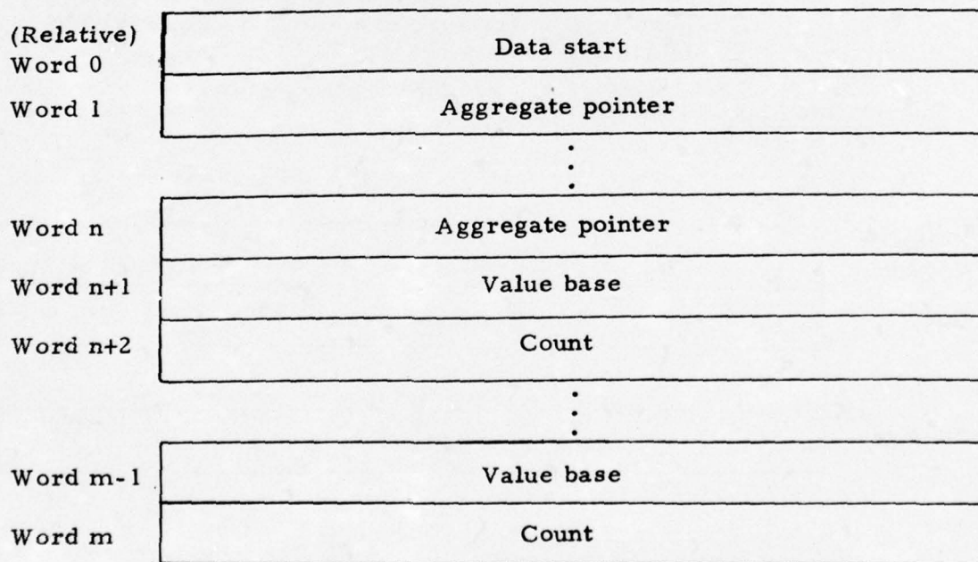
Figure 52. GRMAP Data Set Node Description.
