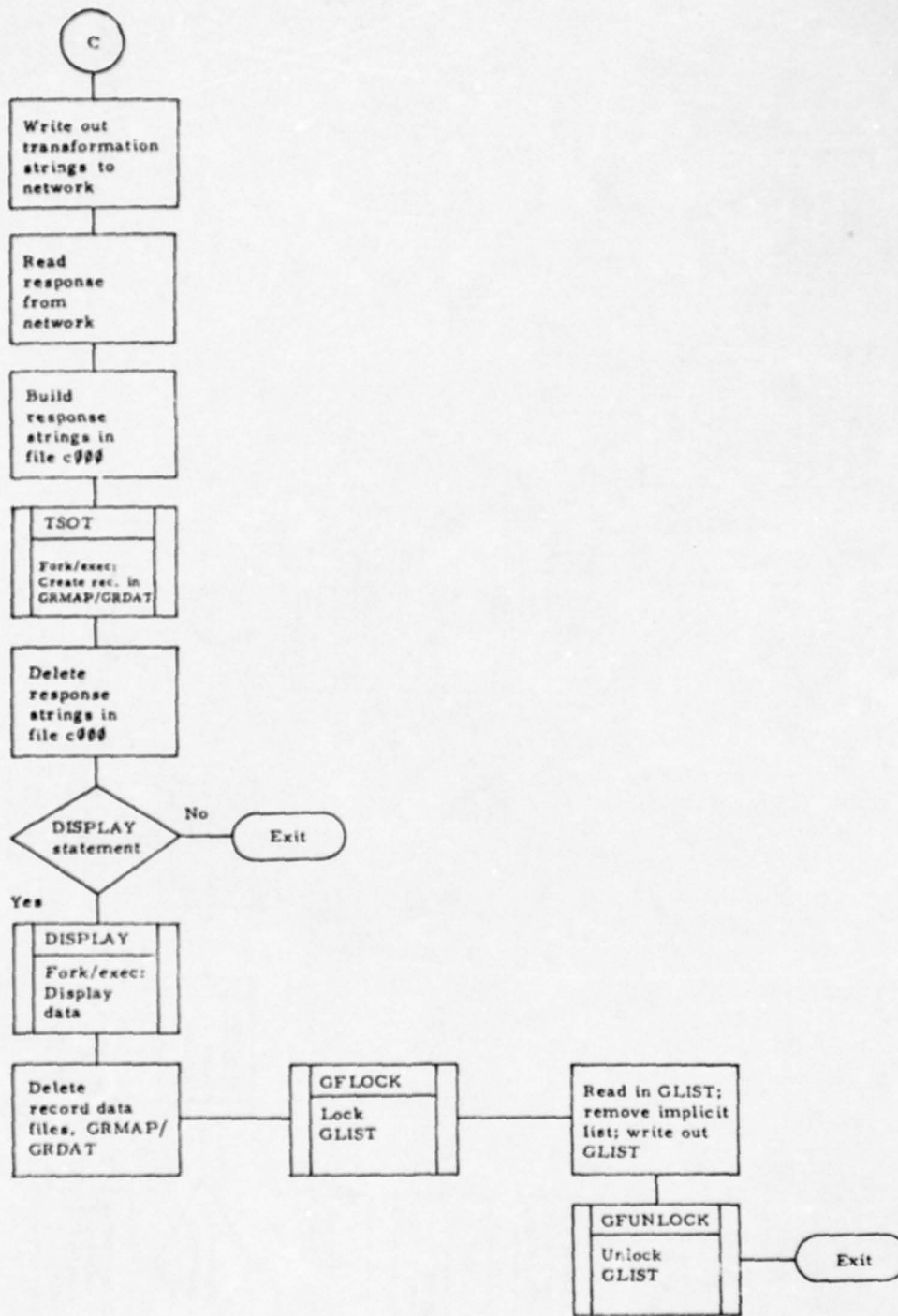
Figure 40. TSIGI Process Data Flow (Sheet 3 of 5).
