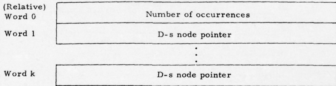
Figure 53. GRMAP Occurrence Node Description.
