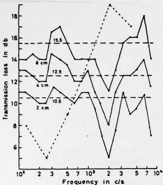
Figure 4. Transmission loss of compact snow (density 0.35, air flow resistance 14.0 g/s·cm 3 ). The horizontal broken lines are the entire characteristics of white noise while the dotted line is the transmission loss in the air of a pumice block 10.2 cm thick with two holes.
