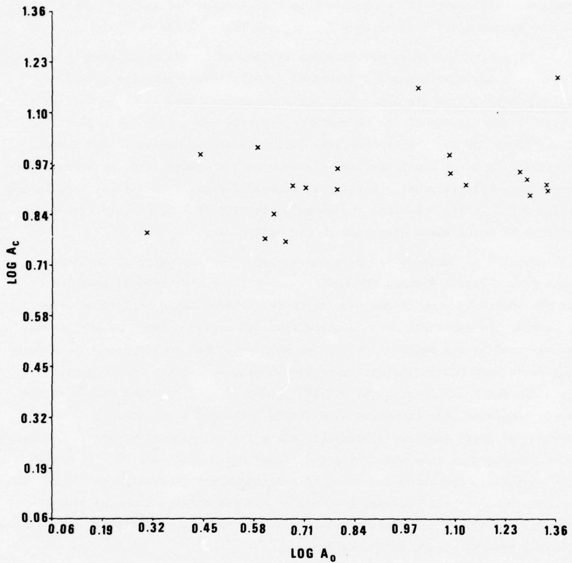
Figure 21. \text{Log } A_c versus \text{log } A_0 for event 7.
