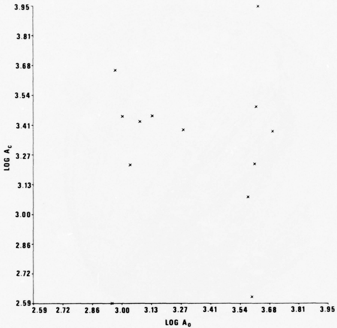
Figure 11. \text{Log } A_c versus \text{log } A_0 for event 2.
