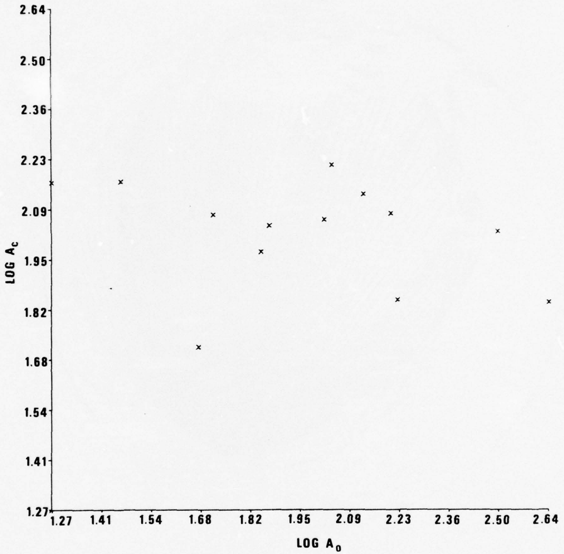
Figure 17. Log A c versus log A 0 for event 5.
