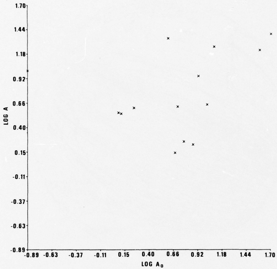
Figure 15. \text{Log } A_c versus \text{log } A_0 for event 4.
