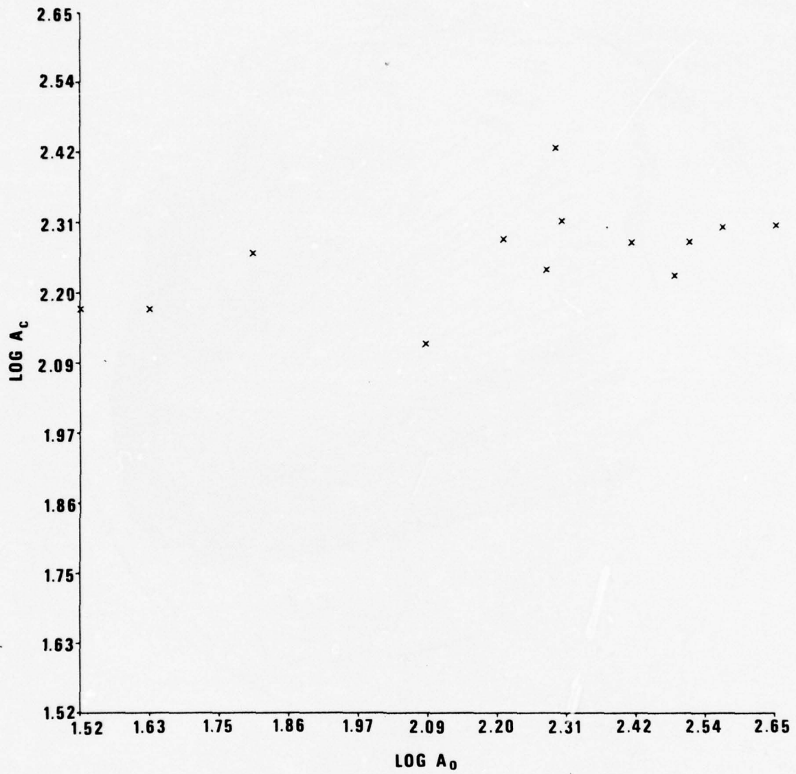
Figure 19. \text{Log } A_c versus \text{log } A_0 for event 6.
