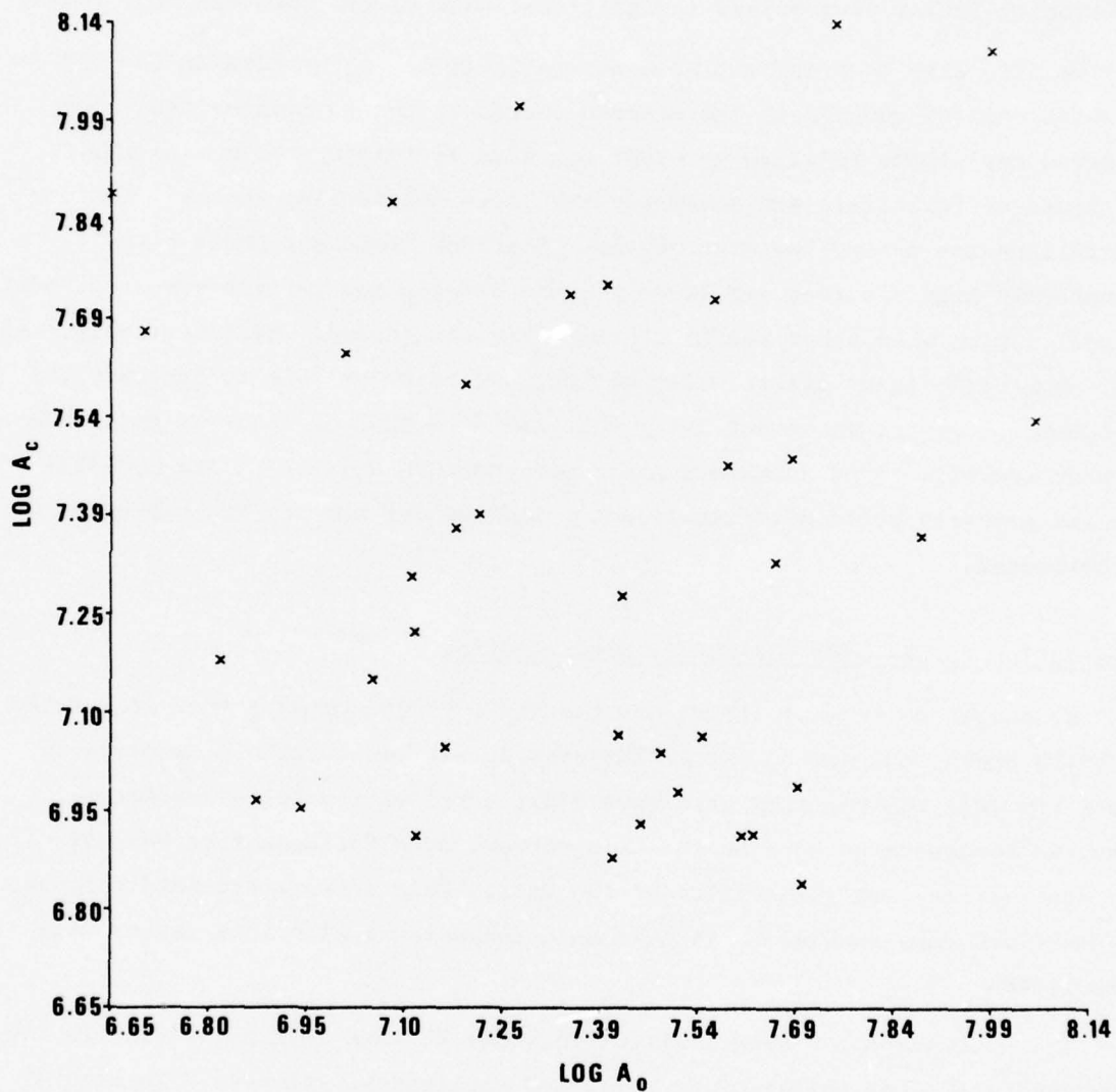
Figure 7. \text{Log } A_c versus \text{log } A_0 for LONGSHOT/MILROW/CANNIKAN - North American data.
