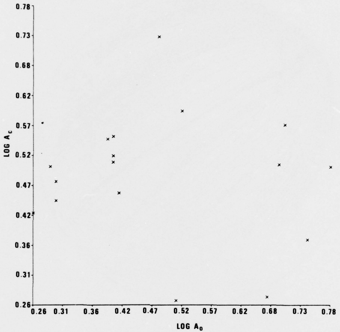
Figure 9. Log A c versus log A 0 for event 1.
