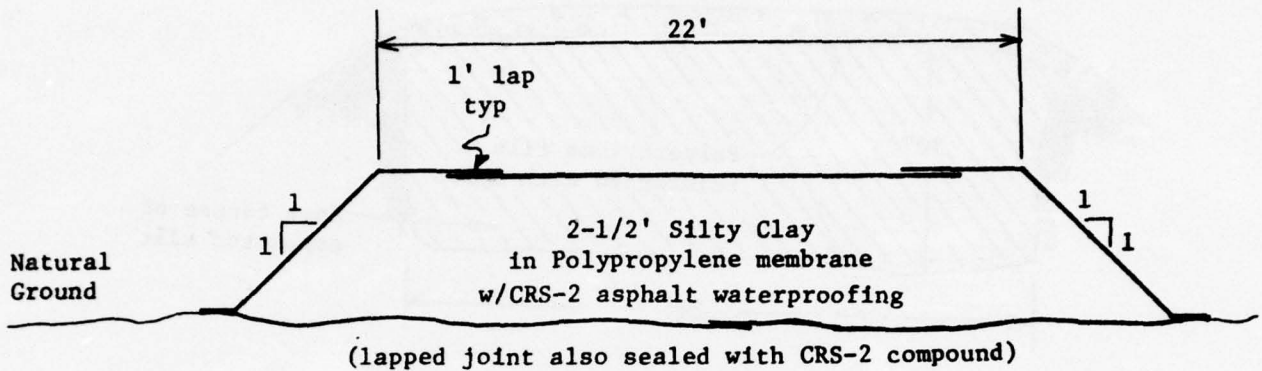
Figure 10. Schematic MESL cross section.
