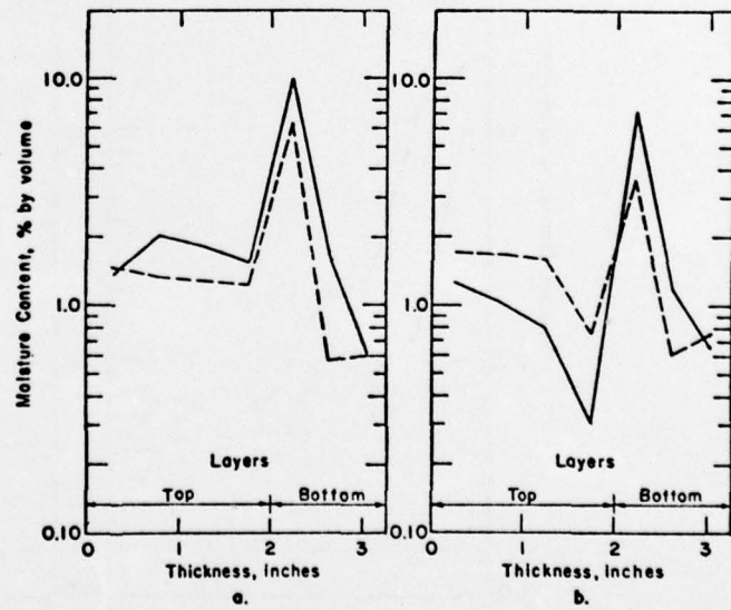
Figure A8. Moisture content of roof at CRREL, Hanover, N.H. (by roof drain).
