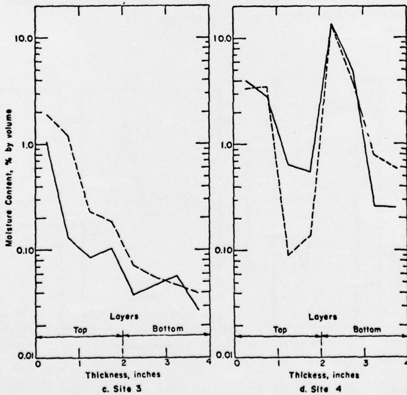
Figure A4. Moisture content of roof of Building 1053, Ft. Wainwright, Alaska.
