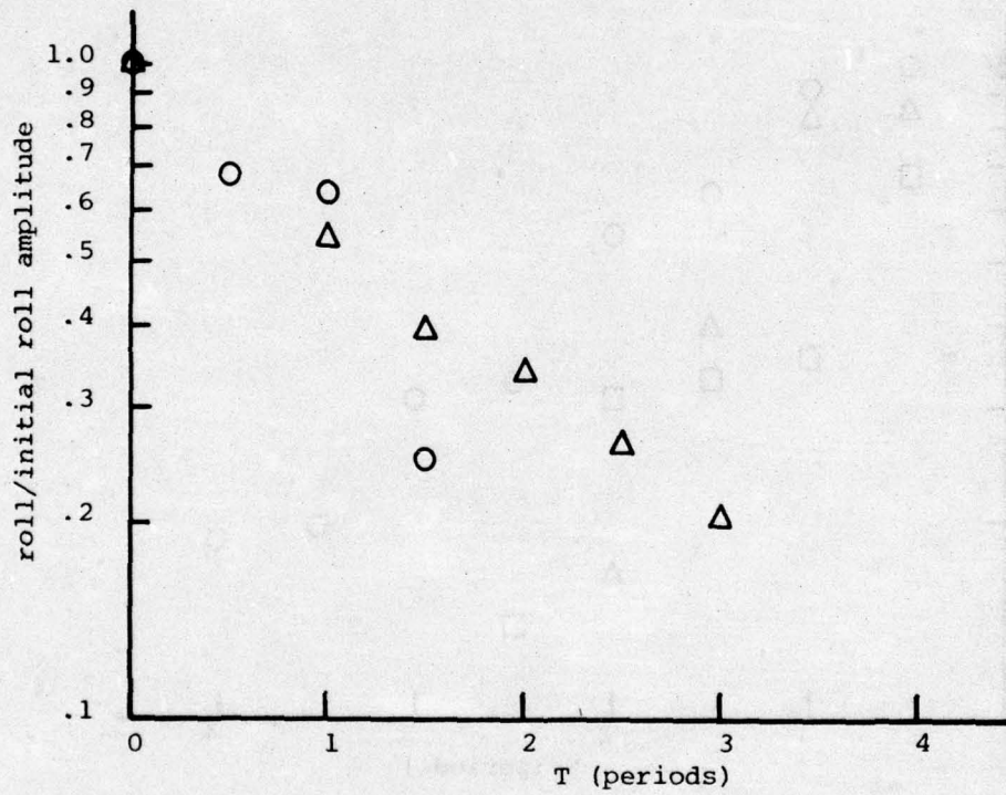
Fig. B.5 Comparison of roll angle transient, full scale and model, jon boat, Test No. 15
