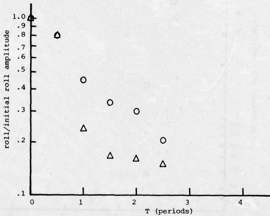
Fig. B.9 Comparison of roll angle transient, full scale and model, runabout, Test No. 9
