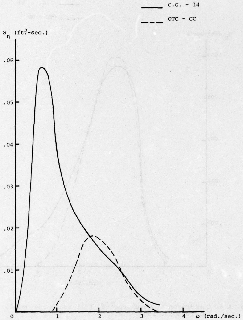
Fig. A.5 Comparison of wave spectra, full scale and model, for Test No. 14
