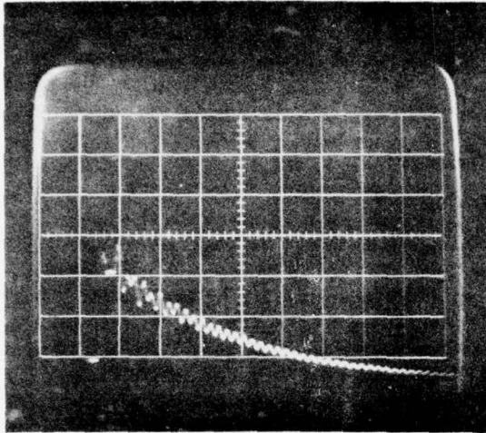
Figure 12. Typical pulse from e-field sensor for simulator EMP measurements. Scale: 1 V/vertical division 200 nsec/horizontal division
