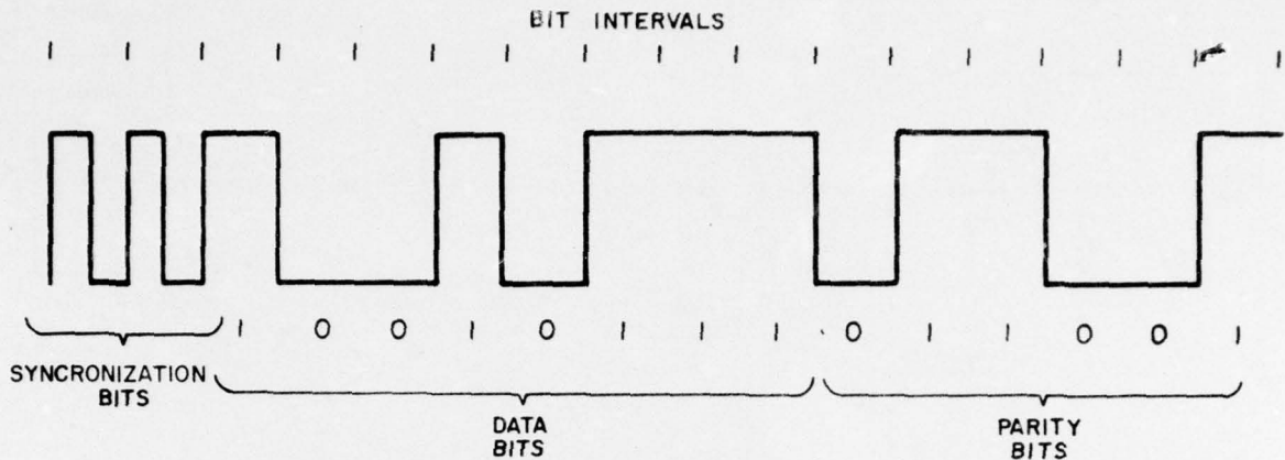
Figure 2. NRZ data and synchronization bits in word format.
