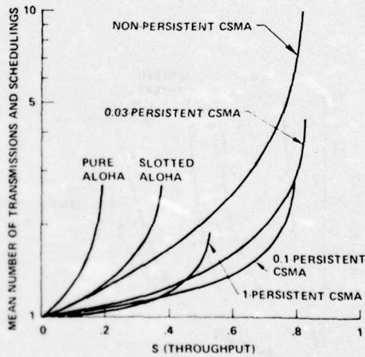
Fig. 7.3—CSMA vs pure and slotted ALOHA: G/S vs throughput ( a = 0.01 ) [Tobagi, 1974, p. 81]
