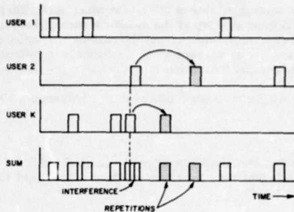
Fig. 4.1—Pure ALOHA Random Access: an example [Abramson, 1973b, p. 510]*
