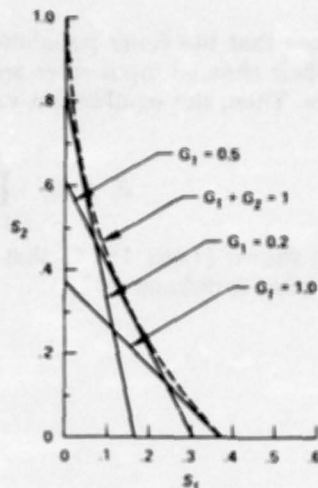
Fig. 5.7—Slotted ALOHA: allowable throughput rates for the large user model [Lam, 1974, p. 63]
