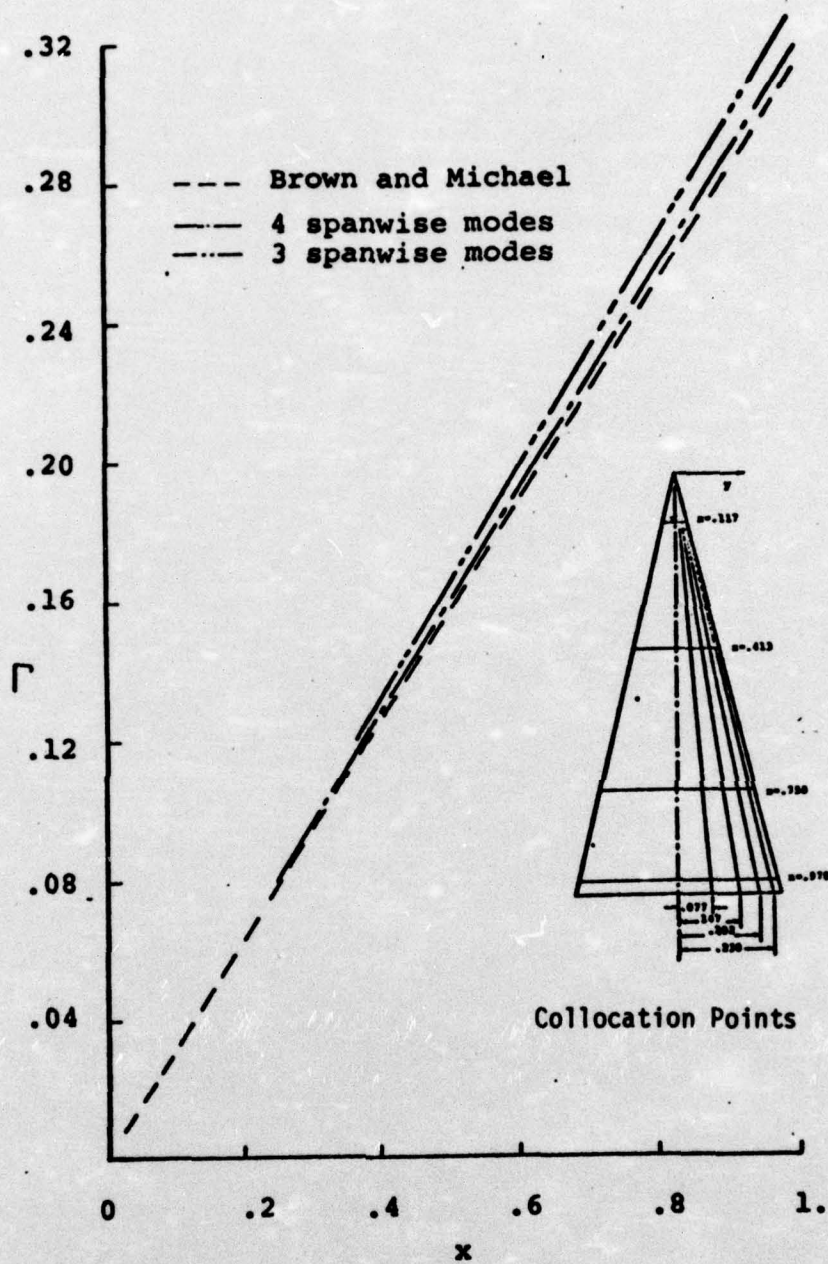
Figure 11. Leading-edge vortex strength for 3 and 4 spanwise modes.
