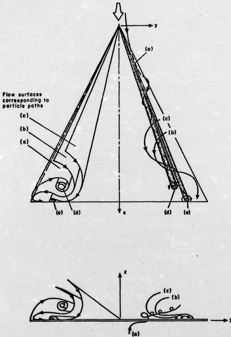
Figure 1. Schematic sketches showing flow on suction side of 70° flat plate delta wing at \alpha=15^\circ [after Örnberg (1954)].
