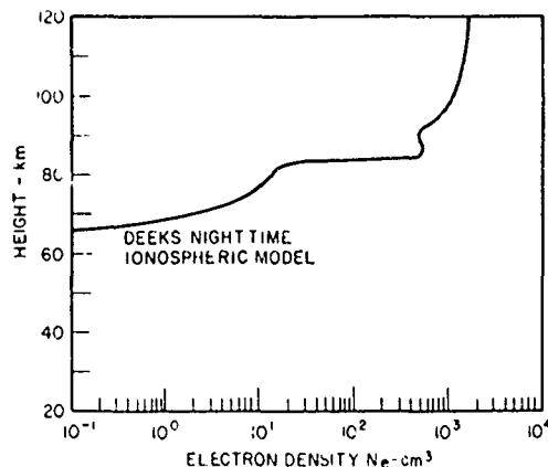
Fig. 2—Ionospheric electron density profile (From Fig. 22, Terrestrial Propagation of Long Electromagnetic Waves, by J. Galejs, Peragmon Press, Copyright 1972 by J. Galejs; used by permission.)
