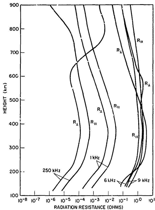
Fig. 12—Radiation resistances of a 100-m radius loop at several frequencies and heights in the ionosphere, and for loop dipole orientations parallel ( R_{\parallel} ) and perpendicular ( R_{\perp} ) to the earth's magnetic field. Values of R_{\perp} were used in computing Tables 1 through 4.
