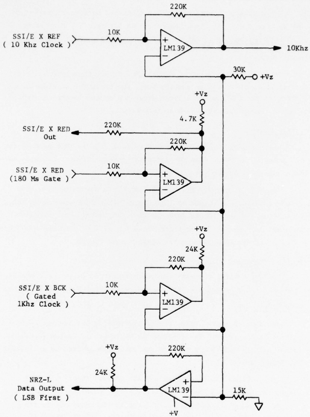
Figure I Interface Buffers
