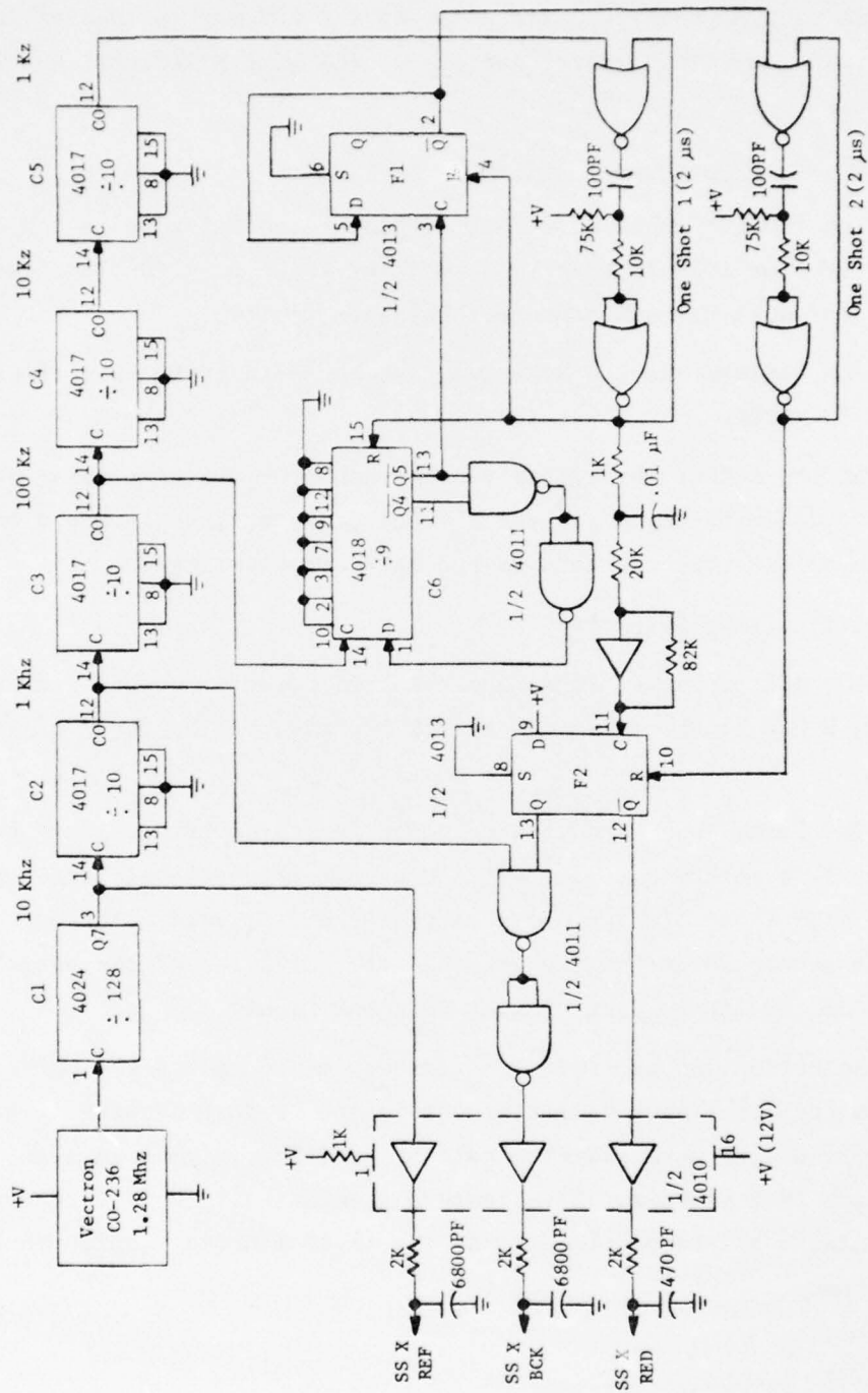
Figure III Signal Simulator
