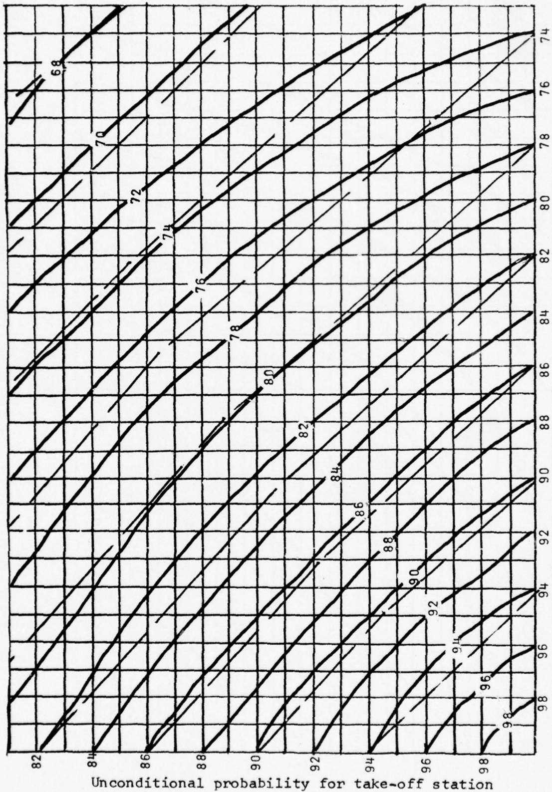
Fig. 5d. Graph of CMSI_t (heavy curved lines) for landing station one hour later for Travis-Alameda, Hill-Mt. Home, Eielson-Elmendorf, Rota-Torrejon, Moron-Torrejon, Moron-Torrejon and Torrejon-Moron comprising the distance interval of 200-300 miles for all months of the year. The dashed lines pertain to CMSI_t . The numbers along the coordinate axis pertain to either set of CMSI values.
