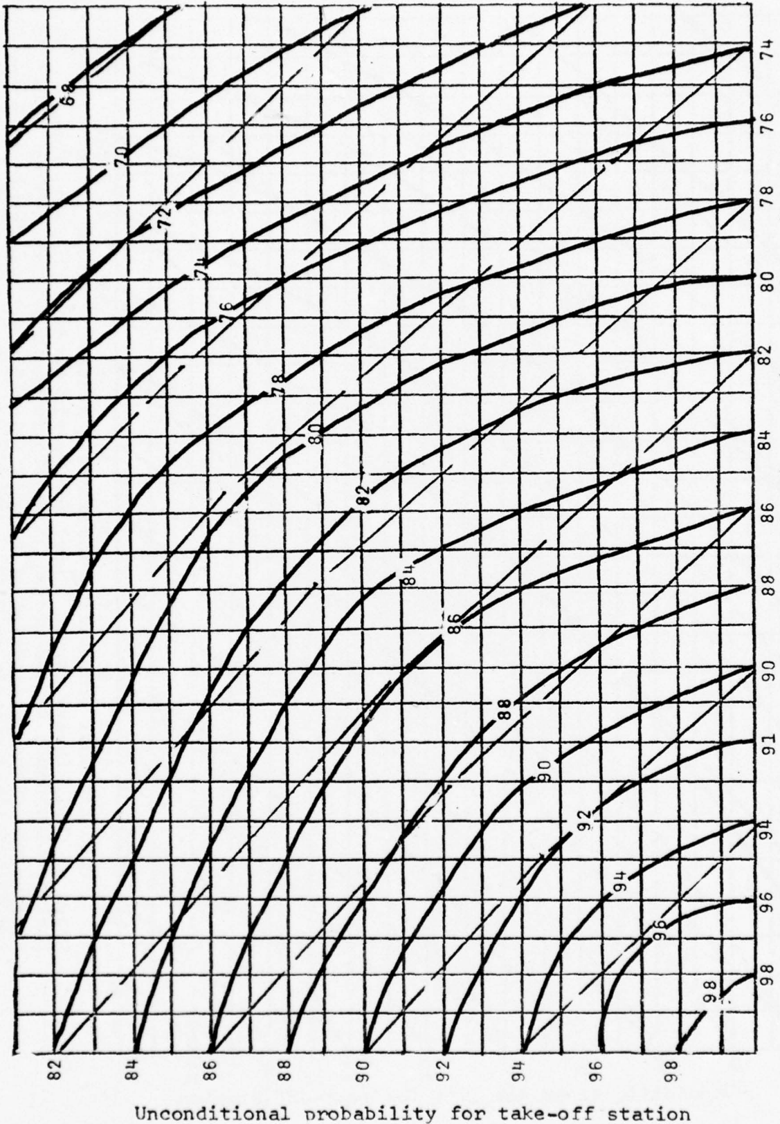
Fig. 5c. Graph of CMSI t (heavy curved lines) for Pope-Charleston, S.C., Charleston-Robins, Robins-Dobbins, Benning-Robins, Ft. Hood-Bergstrom, Altus-Tinker, and Dobbins-Robins comprising the distance interval of 100-200 miles for all months of the year. The dashed lines pertain to CMSI i . The numbers along the coordinate axis pertain to either set of CMSI values.
