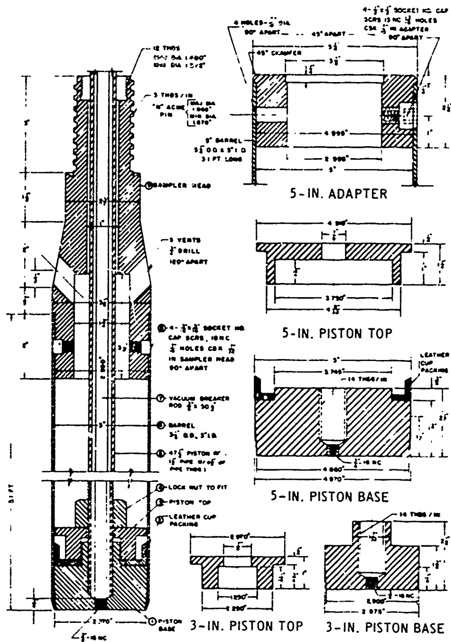
Figure 11. Hvorslev-type 3-in.-diameter fixed-piston sampler with 5-in. adapter. (U. S. Army Engineer Waterways Experiment Station drawing No. 1295-3, revised 9 Oct 53)
