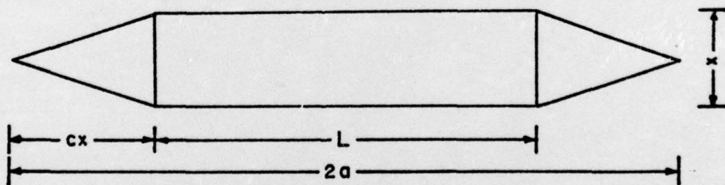
FIGURE 32. SHORT, FULL-VOLUME VGRB (1/4 SCALE)
