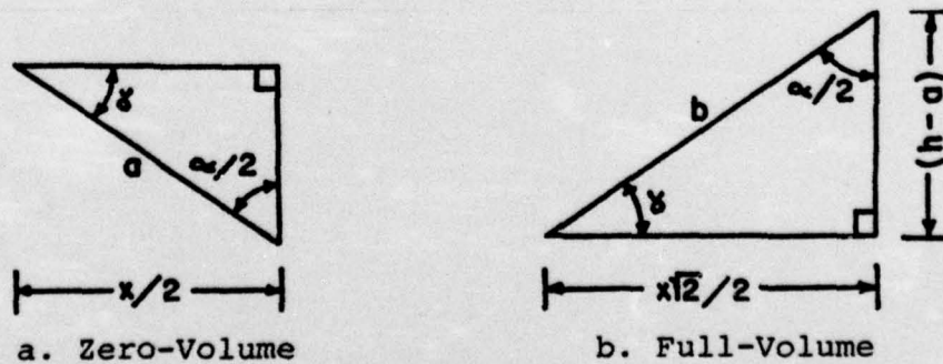
FIGURE 29. VGRB END SECTION DIMENSIONAL RELATIONSHIP TRIANGLES
