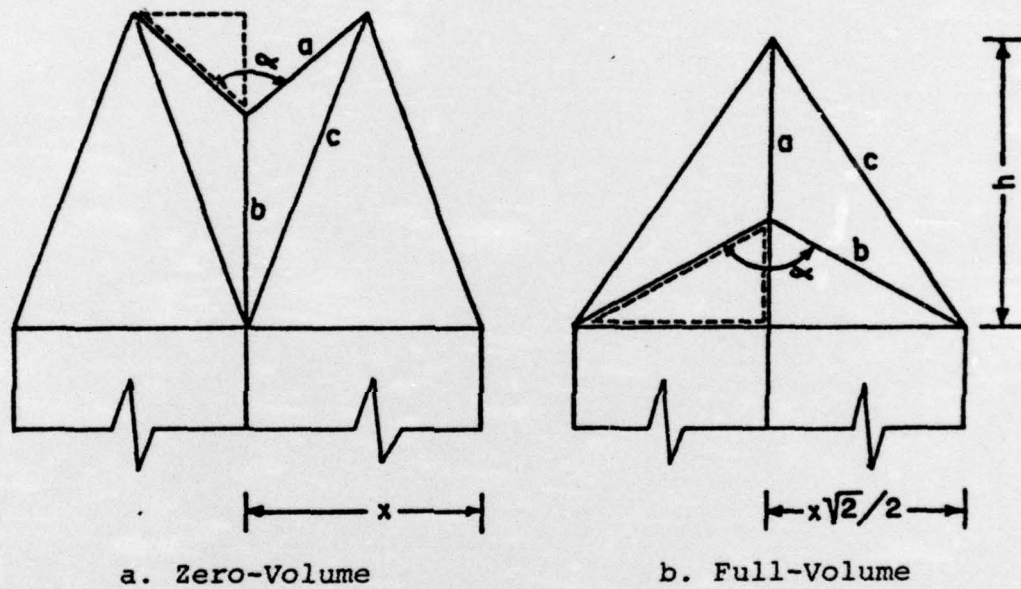
FIGURE 28. VGRB END SECTION DIMENSIONAL PARAMETERS
