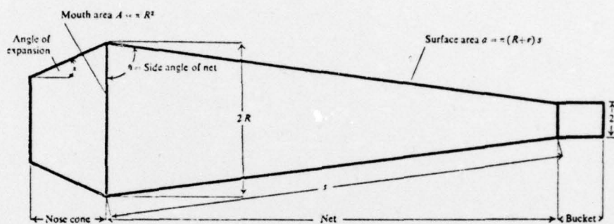
Figure 1. Generalized geometry of a plankton net with a mouth reduction nose cone (From Tranter and Heron, 1967).
