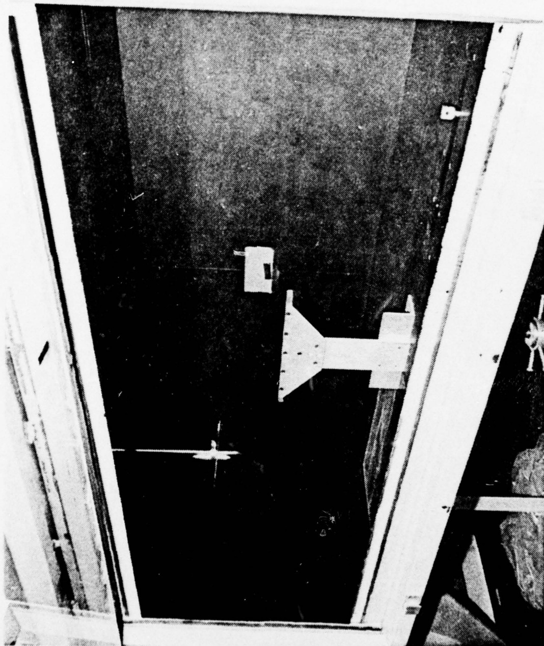
Plate 3. Remote controlled hot-wire anemometer probe.
