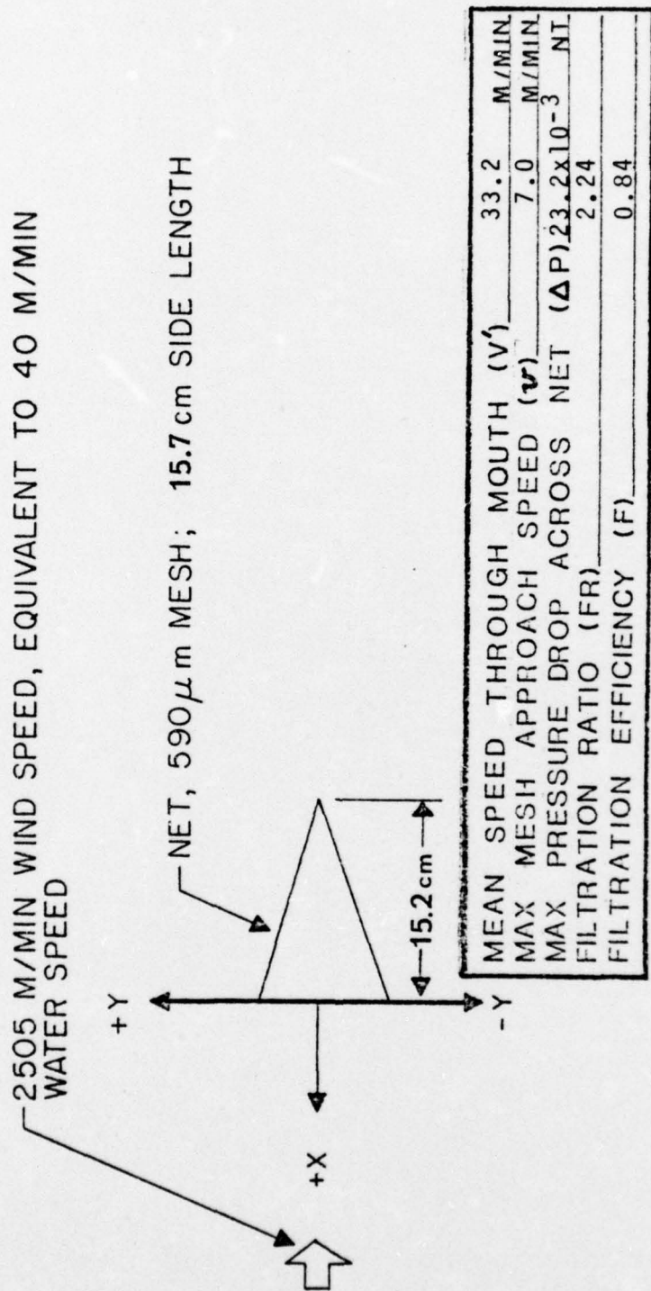
Figure 6. Sampler model A: simple conical net.
