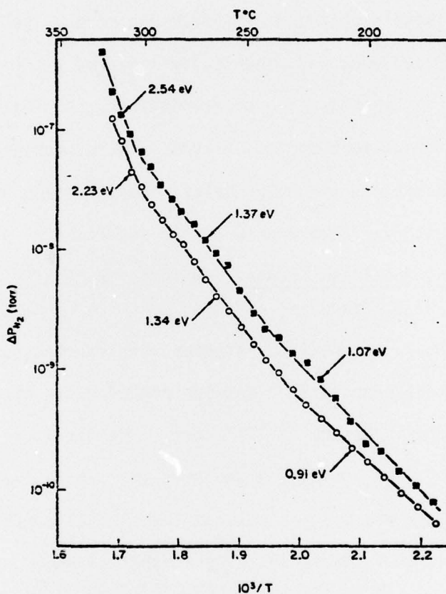
FIG. 1. Temperature dependence of the N_2 partial pressure for a powder sample of KN_2 . ○, run #5; ■, run #12.
