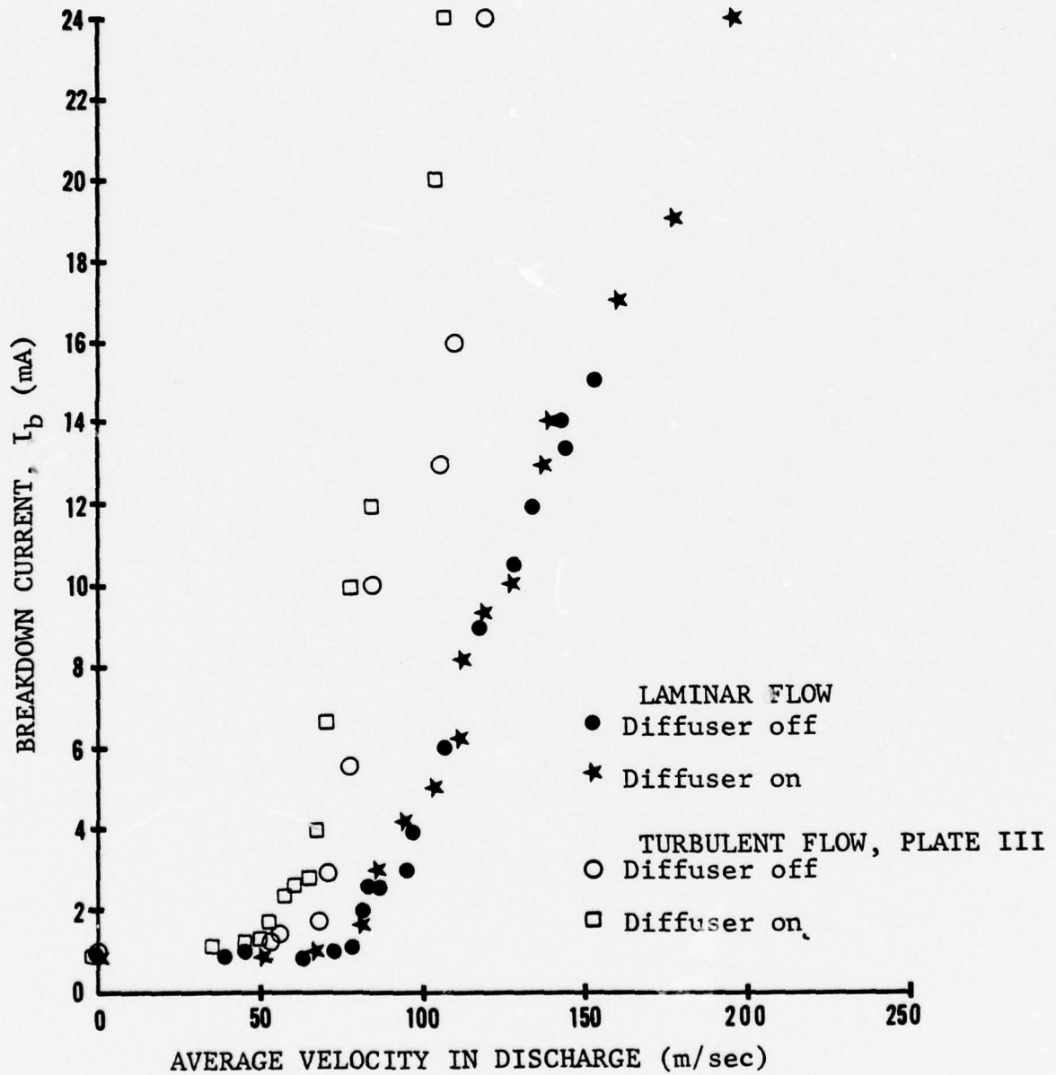
Figure 18. Breakdown Current Versus Average Velocity Through the Discharge
