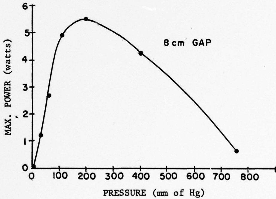
Figure 1. Breakdown Power Versus Pressure (Loeb Data, Ref. 6)
