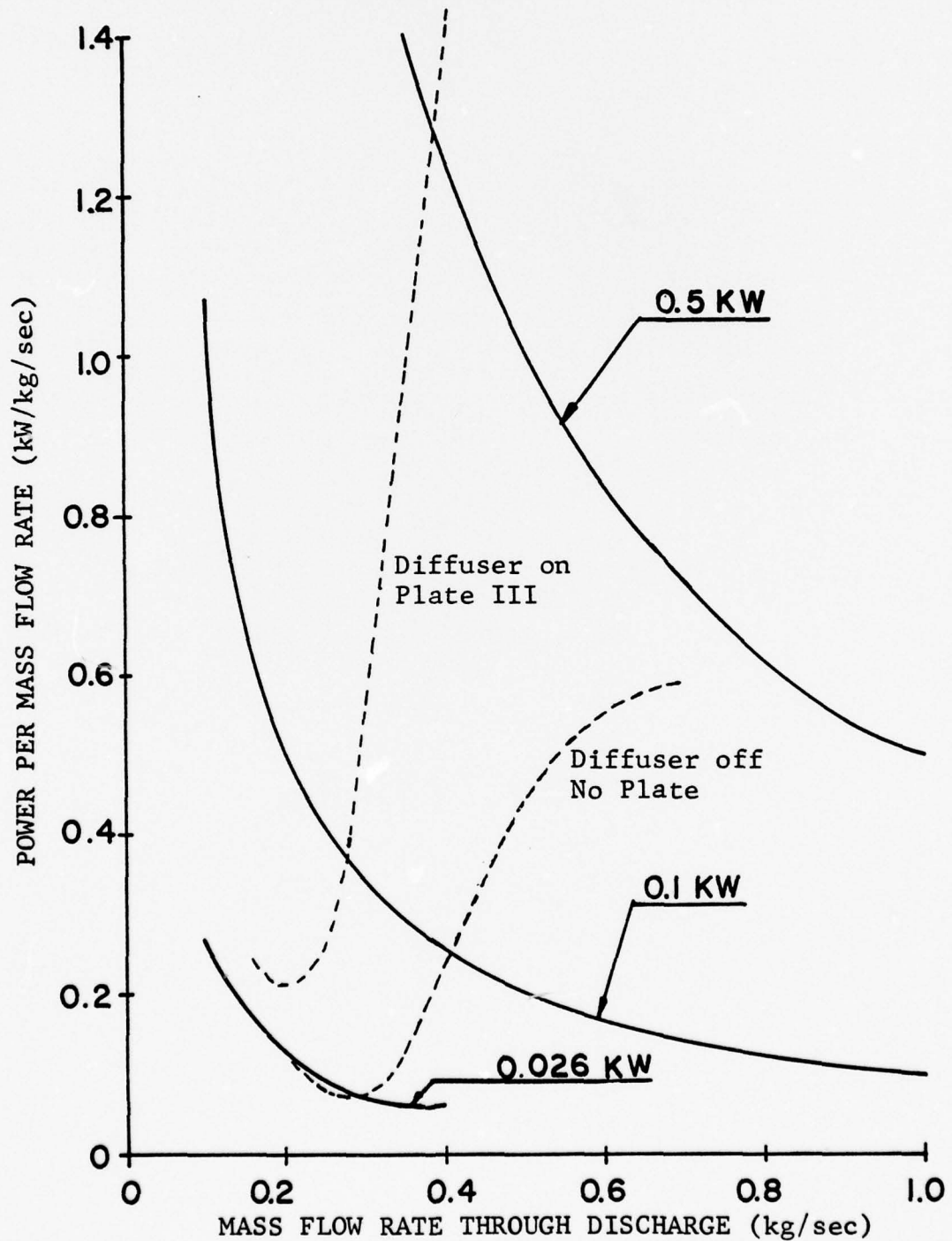
Figure 15. Constant Power Curves
