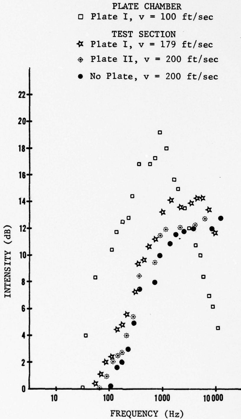
Figure 12. Turbulence Spectra
