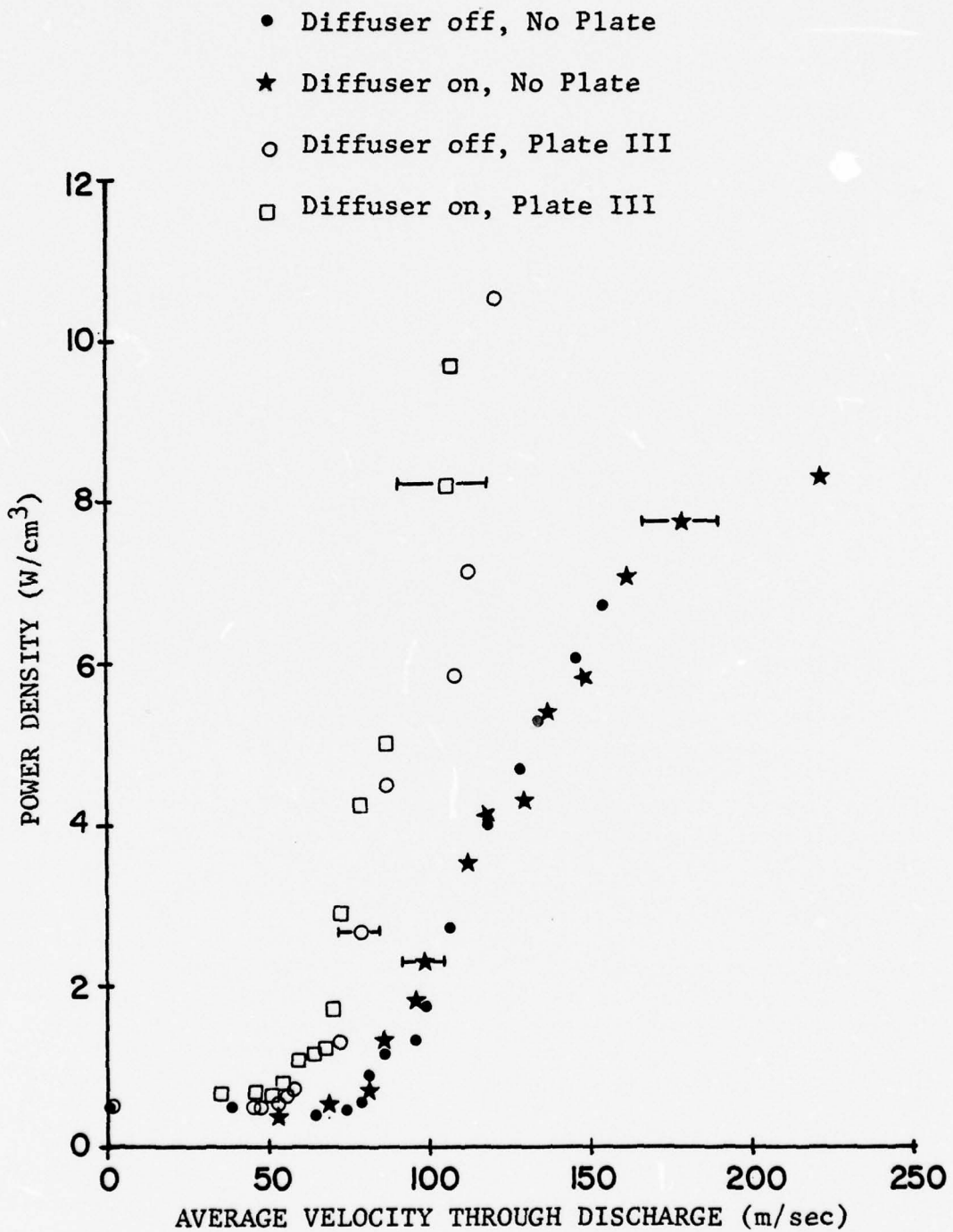
Figure 16. Power Density Versus Average Velocity Through the Discharge
