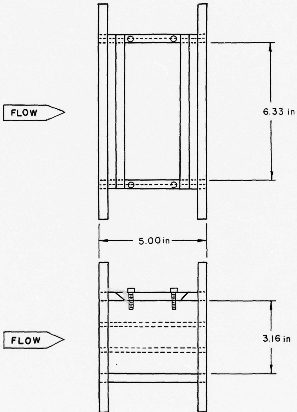
MATERIAL: 0.75 INCH PLEXIGLASS Figure 5. Plate Chamber Schematic
