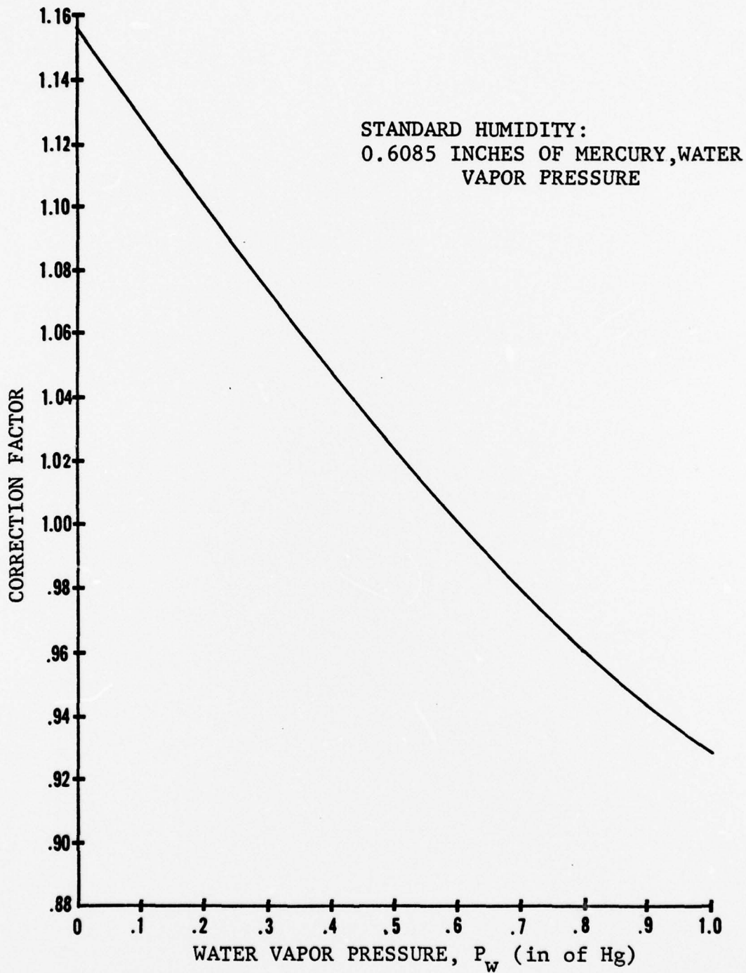
Figure 22. Relative Humidity Correction Curve (Ref. 9)
