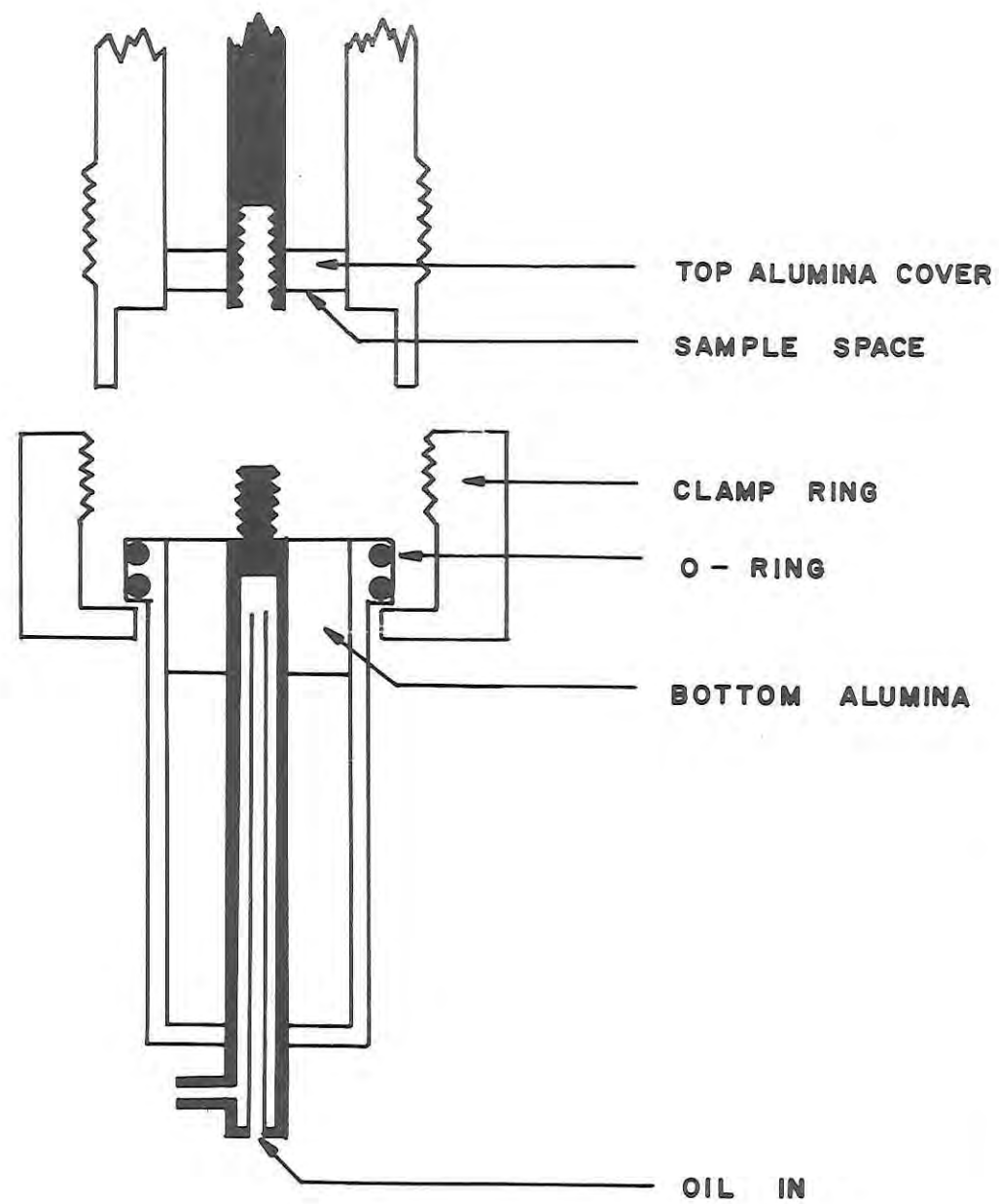
Figure 3: Schematic diagram of the quarter wavelength holder for 900, 300 MHz, 80 to 120°C.
