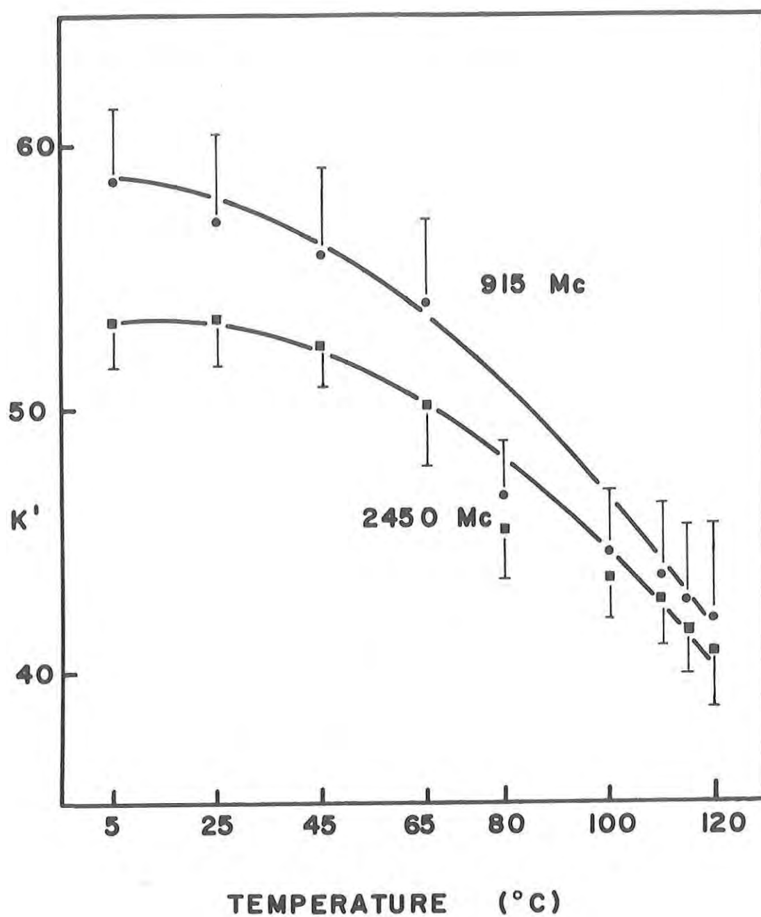
Figure 4: Dielectric constant K' of unsalted meats at 2450 and 915 MHz, 5 to 120 ^{\circ}\text{C} . Mean and standard deviations.
