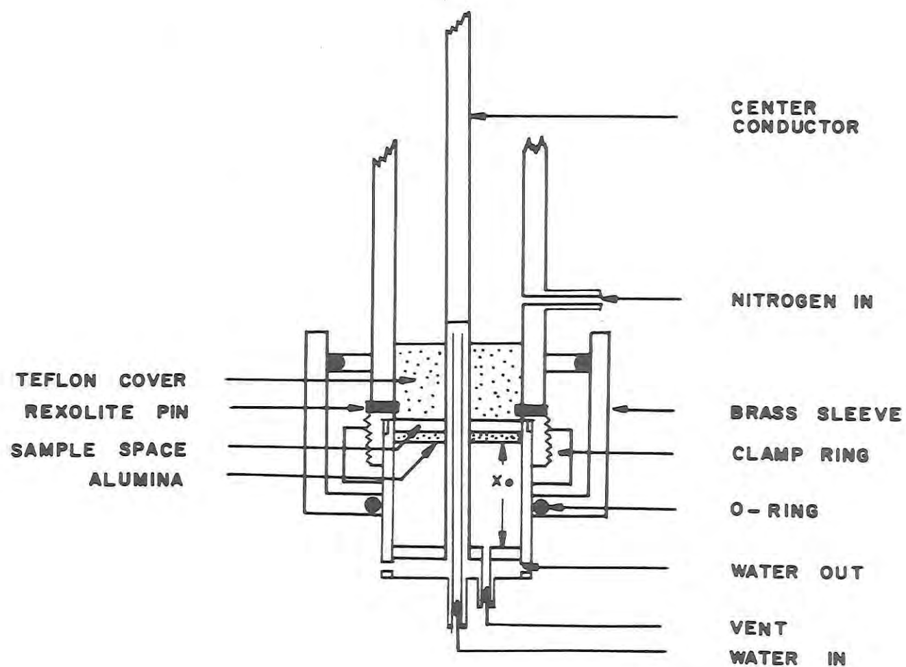
Figure 2: Schematic diagram of the quarter wavelength holder for 2450 MHz, 5 to 65°C.
