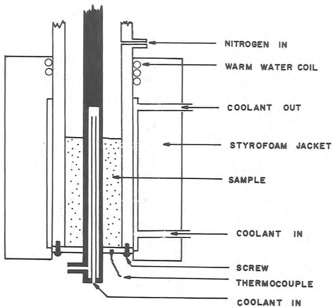
Figure 1: Schematic diagram of the open circulated low temperature holder for all three frequencies.
