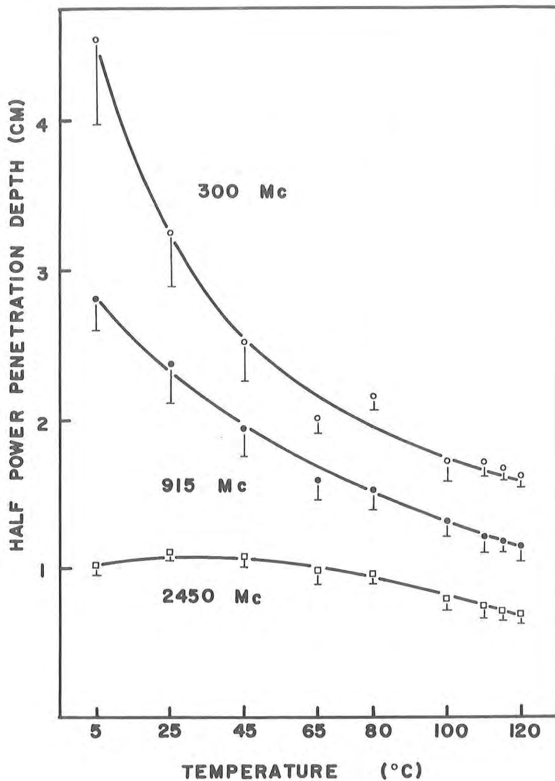
Figure 6: Half Power Penetration Depth of raw unsalted meats at 2450, 915, and 300 MHz, 5 to 120°C. Mean and standard deviation.
