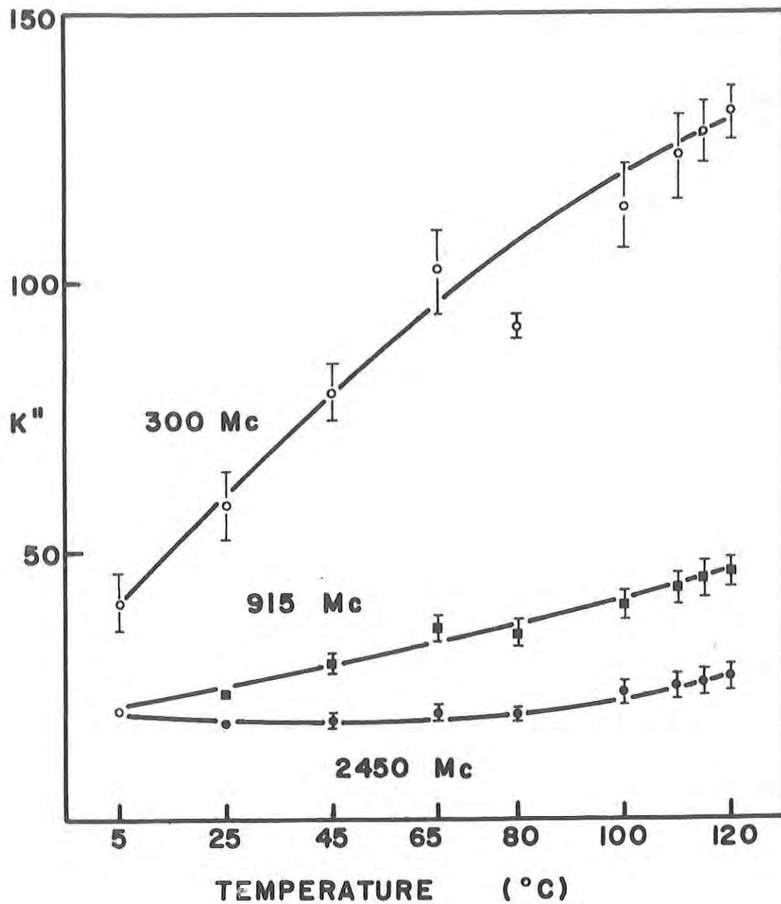
Figure 5: Dielectric loss K'' of unsalted meats at 2450, 915, and 300 MHz, 5 to 120 ^{\circ}\text{C} . Mean and standard deviations.
