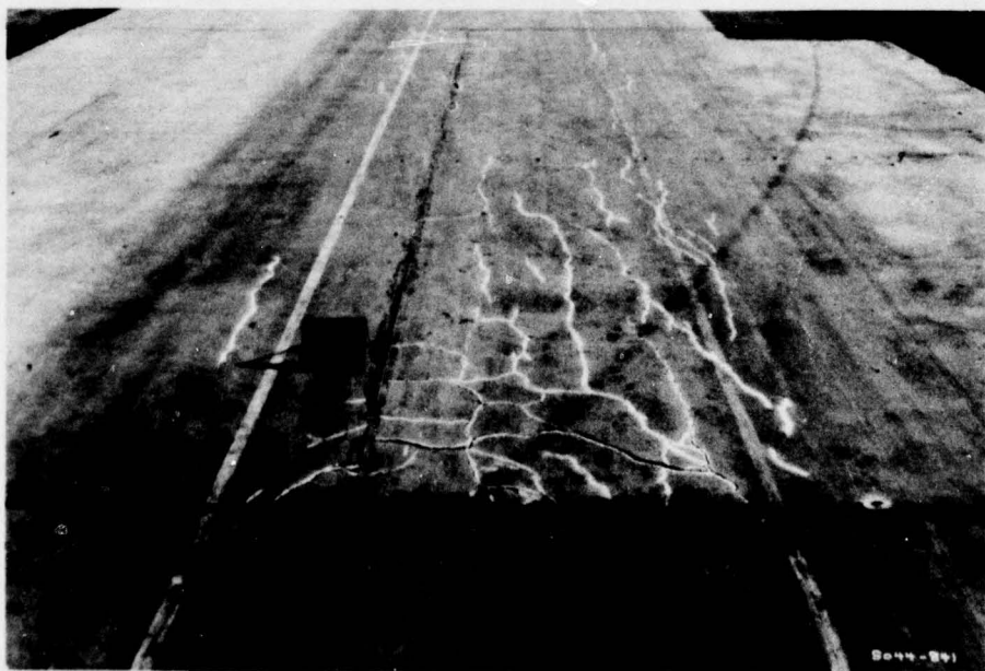
Figure 3-2. Condition of 4-in. fibrous concrete slab on 17-in. cement-treated base after 1000 coverages of simulated B-747 traffic
