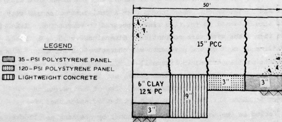
Figure 11-2. Profiles of items in the rigid pavement test section
