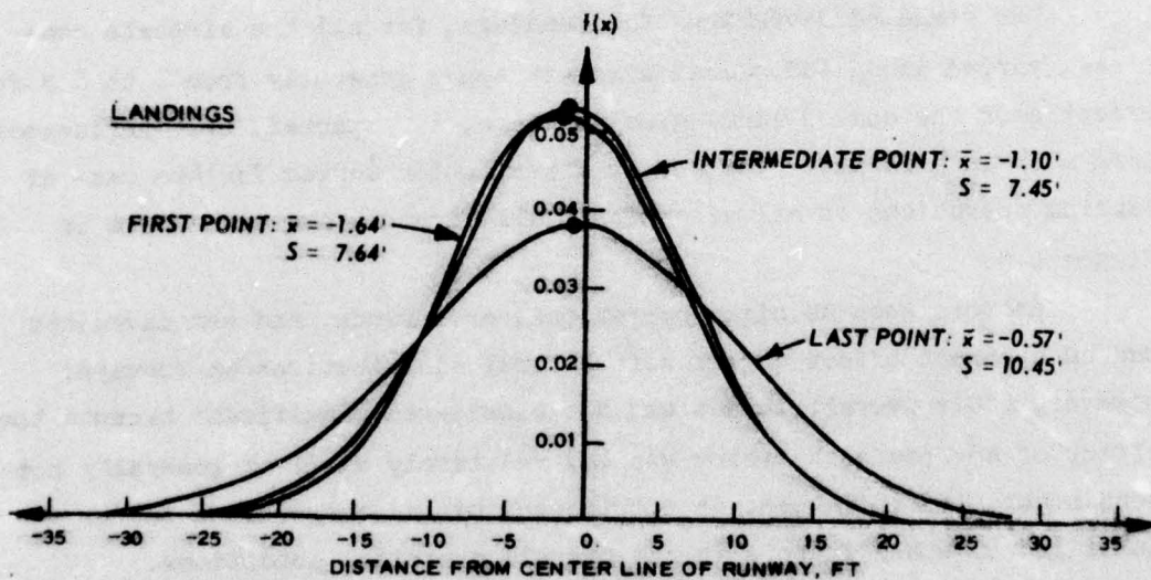
Figure 6-3. Summary of lateral distributions on runways for all aircraft at all airports
