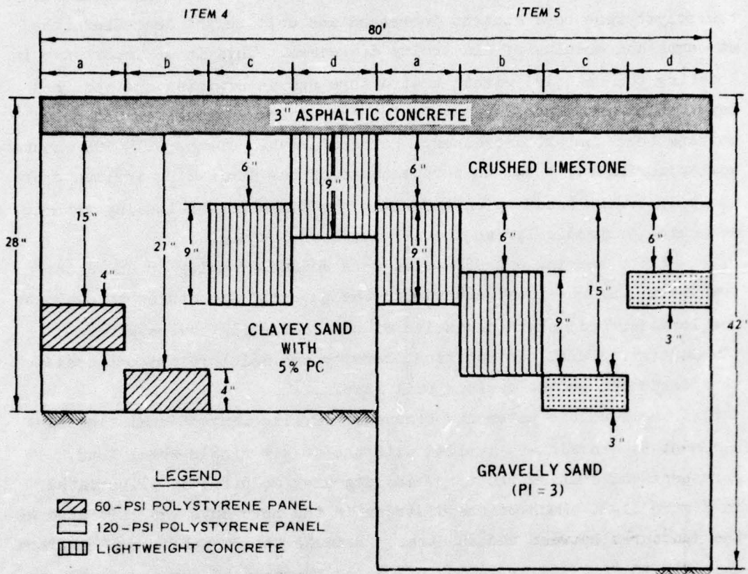
Figure 11-1. Profiles of items in the flexible pavement test section
