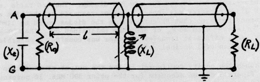
Figure 3. Cavity Spoke Equivalent Circuit
