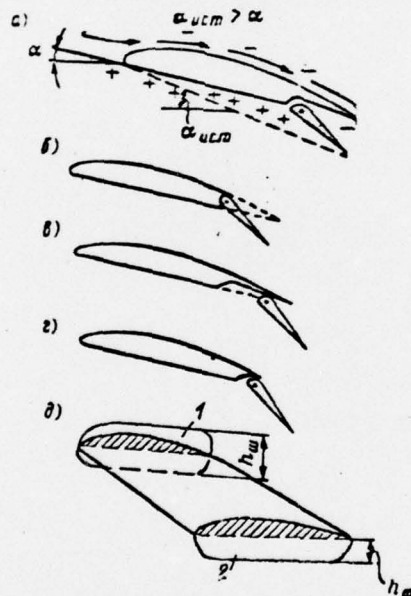
Fig. 14. Systems to increase I of WIG wings. a - flow pattern of a simple flap covered on top; b - simple flap; c - simple flap with a sliding rotating axis; d - slotted flap with a shaped slot; e - end plates: 1 - two-sided; 2 - one-sided.
