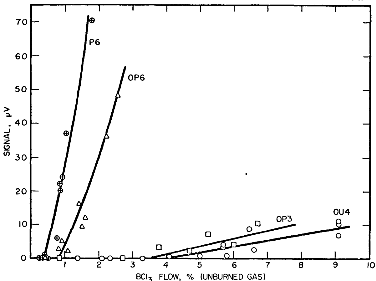
Fig. 4 SCATTERED LIGHT SIGNAL VS. \text{BCl}_3 FLOW
