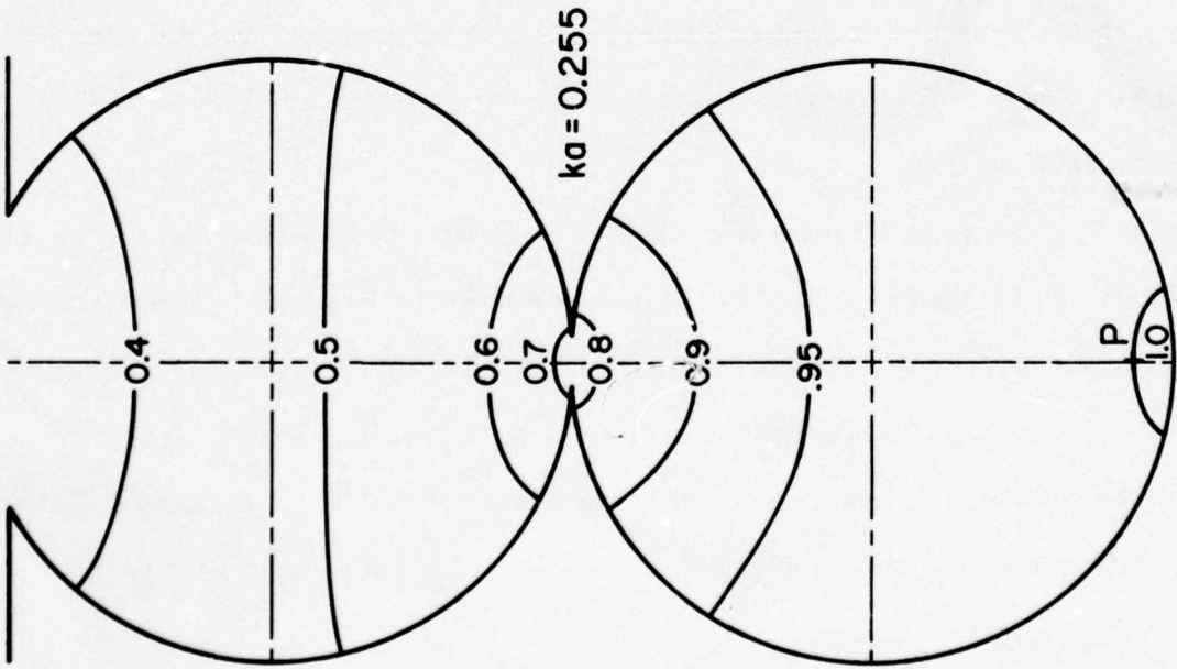
Fig. 18 Shape of Mode 1 ( ka = 0.255 ): Two Coupled Circular Harbors
