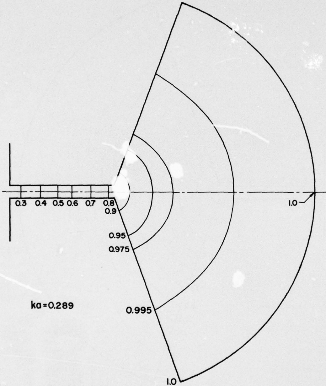
Fig. 37 Shape of Mode 1 for Circular-Segment Harbor; ka = 0.289
