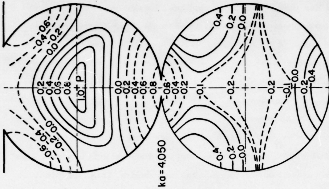
Fig. 24 Shape of Mode 7 ( ka = 3.863 ); Two Coupled Circular Harbors
