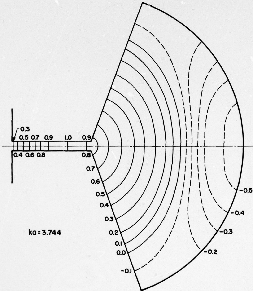
Fig. 38 Shape of Mode 2 for Circular-Segment Harbor; ka = 3.744
