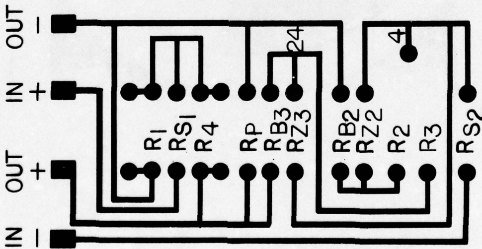
a. Normal Stress Transducers
