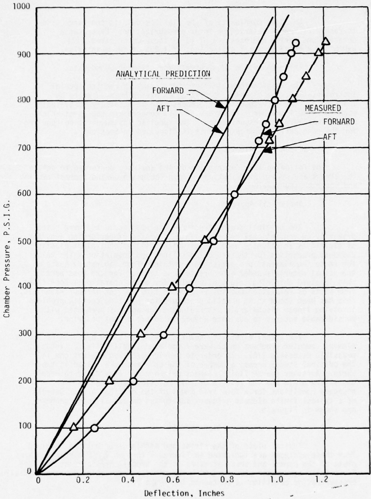
FIGURE 5. LONGITUDINAL DEFLECTION OF BOSSES
