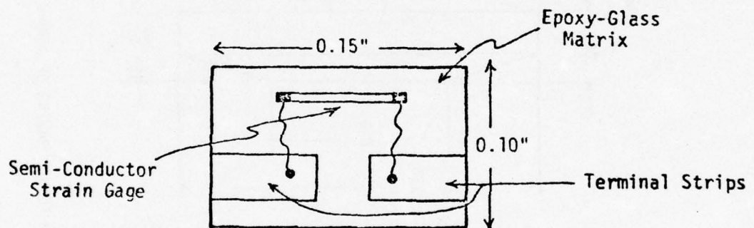
Kulite Ruggedized Strain Gage
