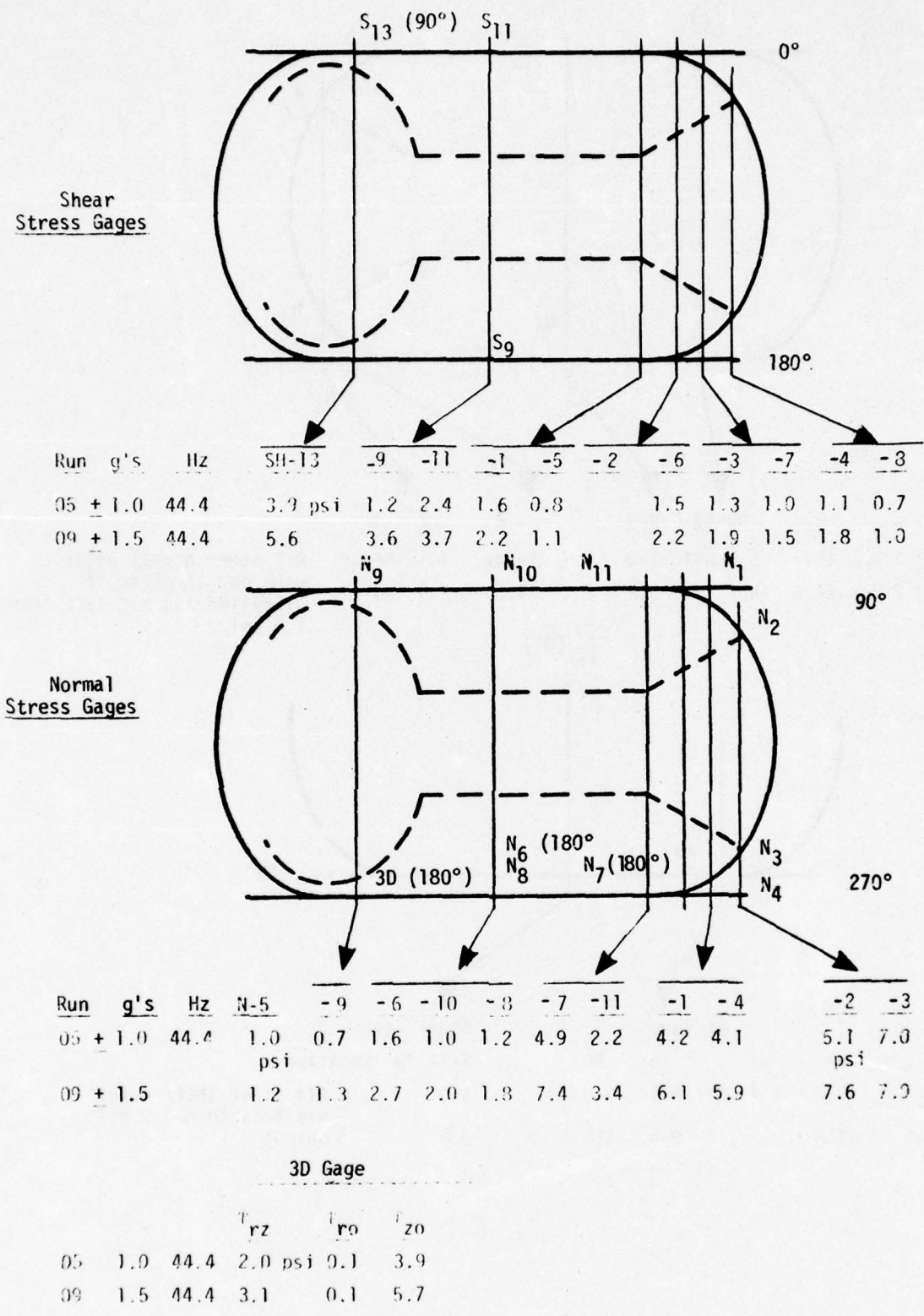
FIGURE 48. DIFFERENTIAL STRESS DATA FROM VIBRATION OF FULL SCALE MOTOR #1 IN THE AXIAL MODE
