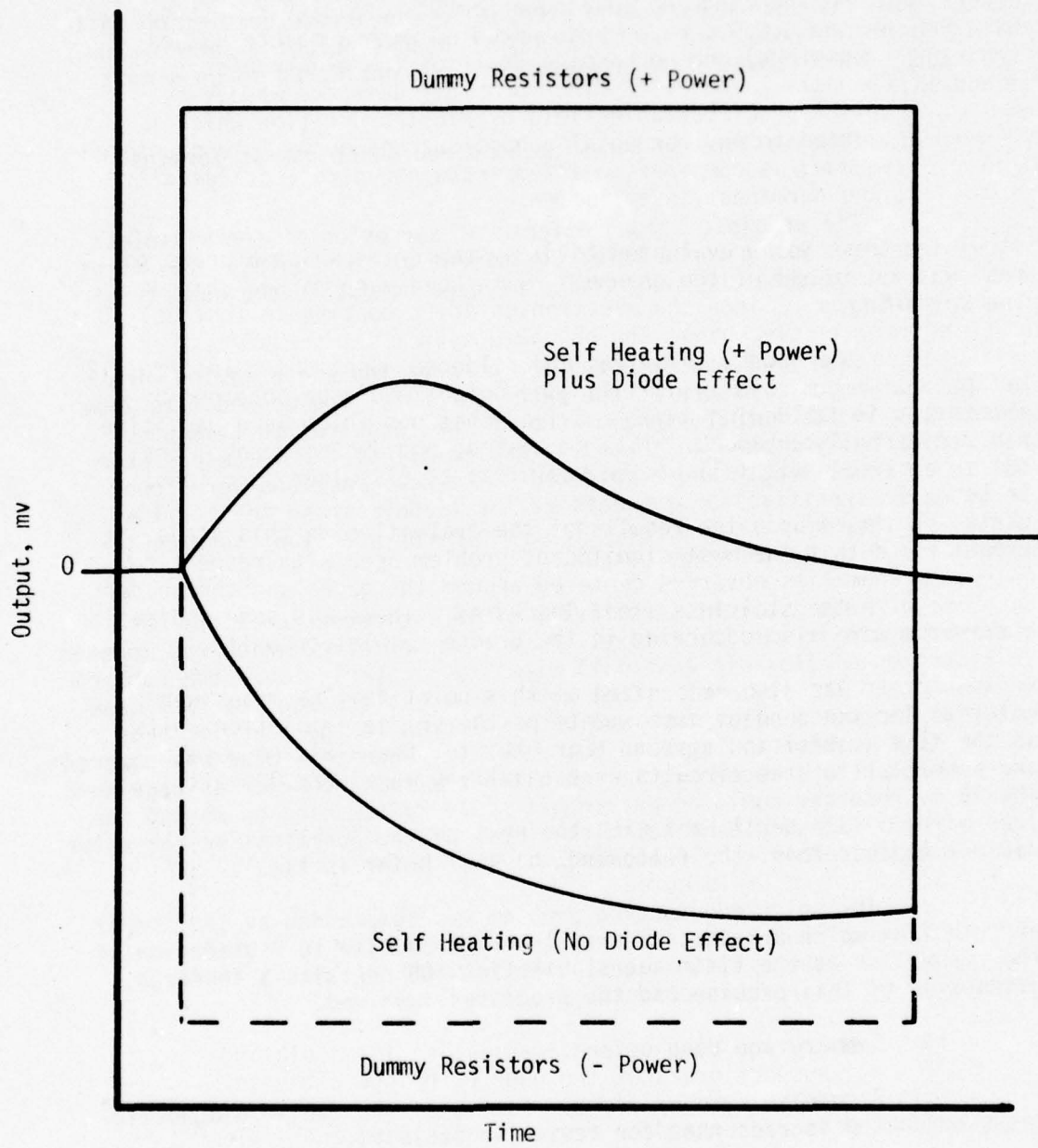
FIGURE 55. SELF HEATING AND DIODE EFFECTS
