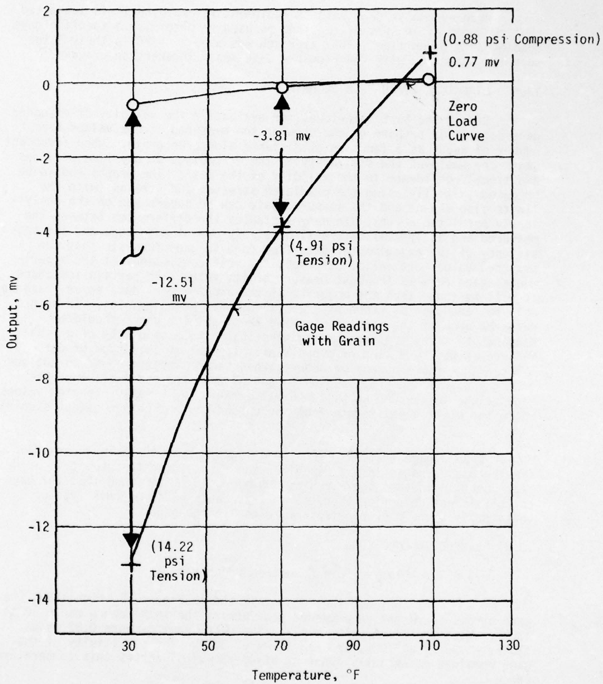
FIGURE 38. TYPICAL THERMAL COOLDOWN TEST DATA FROM EMBEDDED GAGE
