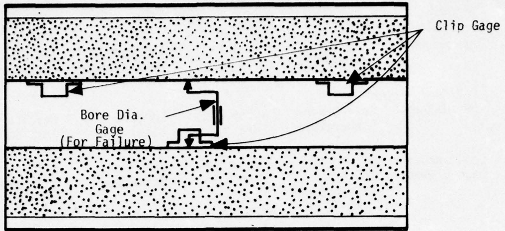
a. Sketch Showing Locations for Strain Gages
