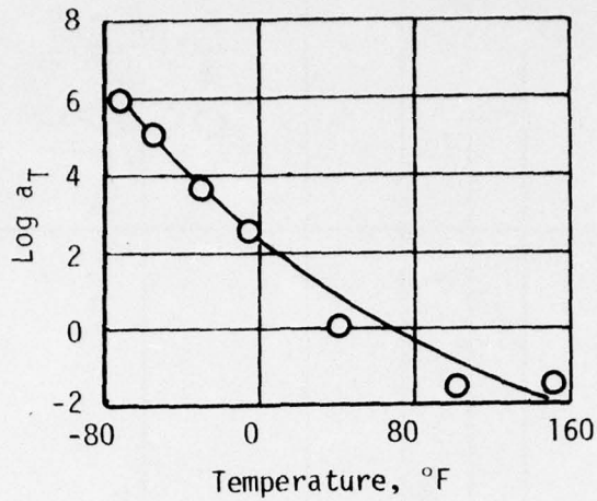
FIGURE 24. TIME-TEMPERATURE SHIFT FACTORS \log a_T VERSUS TEMPERATURE FOR LOCKHEED'S STV PROPELLANT
