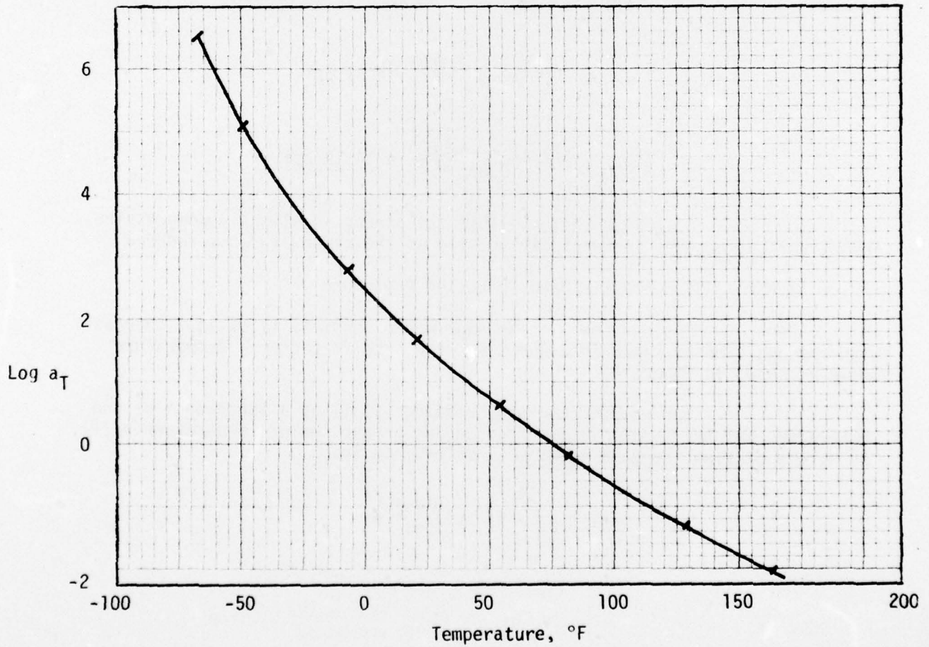
FIGURE 40. LOG a T SHIFT FACTOR CURVE VS TEMPERATURE
