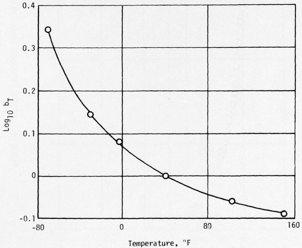
FIGURE 25. VERTICAL SHIFT FACTORS \log b_T VERSUS TEMPERATURE FOR 25 PSI TRANSDUCER
