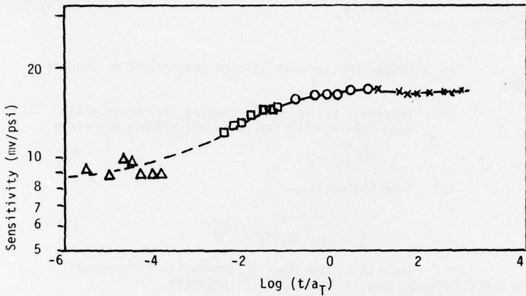
FIGURE 39. MASTER CURVE OF LOG SENSITIVITY VS LOG REDUCED TIME
