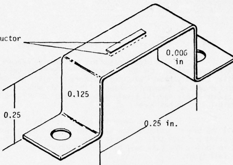
FIGURE 10. CLIP TYPE STRAIN GAGE
