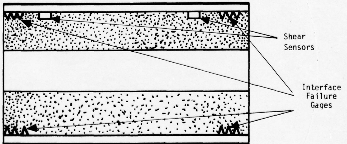
c. Location of Shear Stress Sensors and Failure Gages
