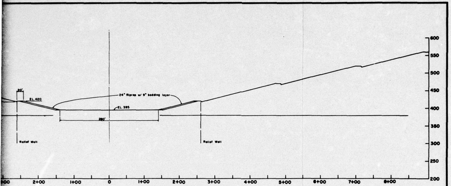
TYPICAL SECTION BETWEEN STA. 12,120+00 AND STA. 13,150+00
