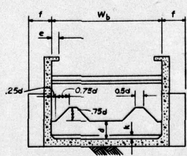
SECTION F-F
