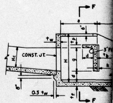
SECTION E-E STILLING BASIN
