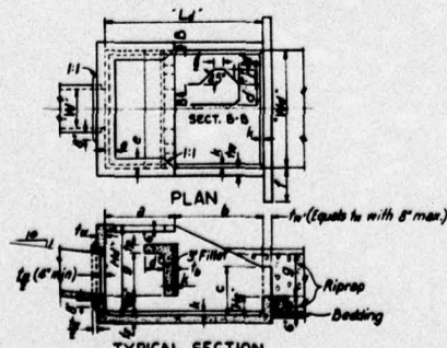
TYPICAL SECTION IMPACT TYPE ENERGY DISSIPATORS FILL SECTION
