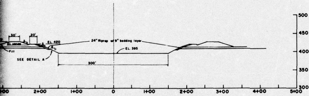
TYPICAL SECTION BETWEEN STA. 13,150+00 AND STA. 13,337+50
