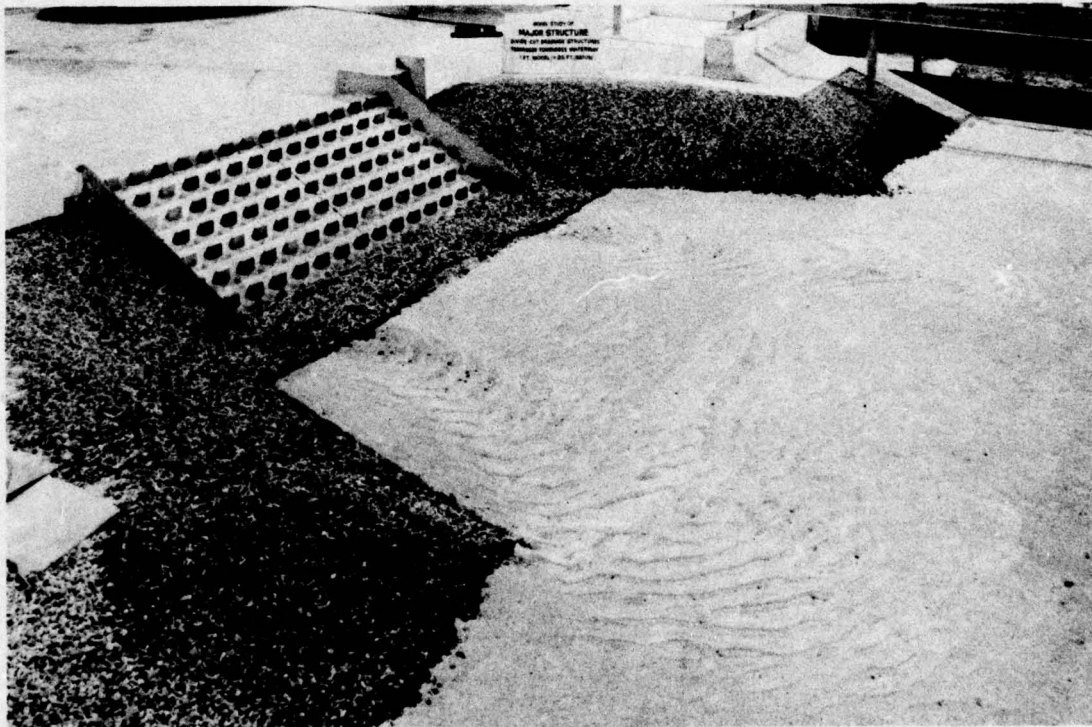
Photo 15. Scour downstream of type 15 structure after 5-hr operation at design discharge 9700 cfs and canal stage 408 (minimum)
