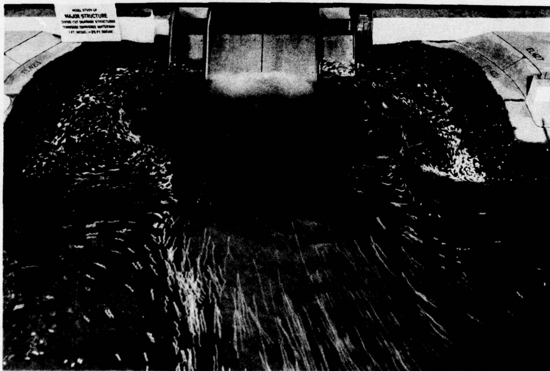
Photo 10. Flow conditions in type 10 stilling basin, discharge 9700 cfs
