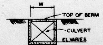
SECTION H-H TYPICAL AT BERM
