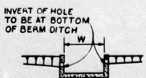
SECTION G-G TYPICAL AT BERM DITCH
