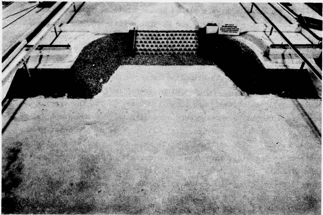
Figure 6. Type 15 (recommended) structure showing stilling pool abutments
