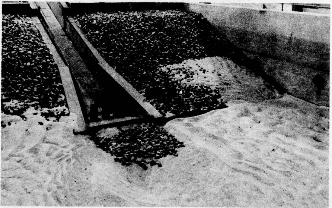
b. Scour after 1-hr operation at design discharge of 900 cfs, with downstream riprap blanket
