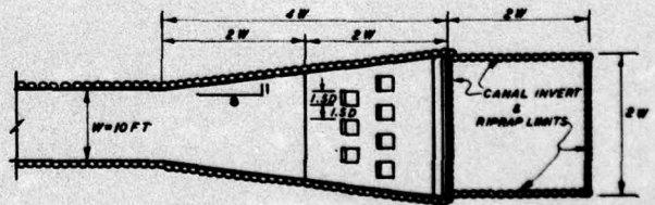
PLAN AT STATION 2+40D
