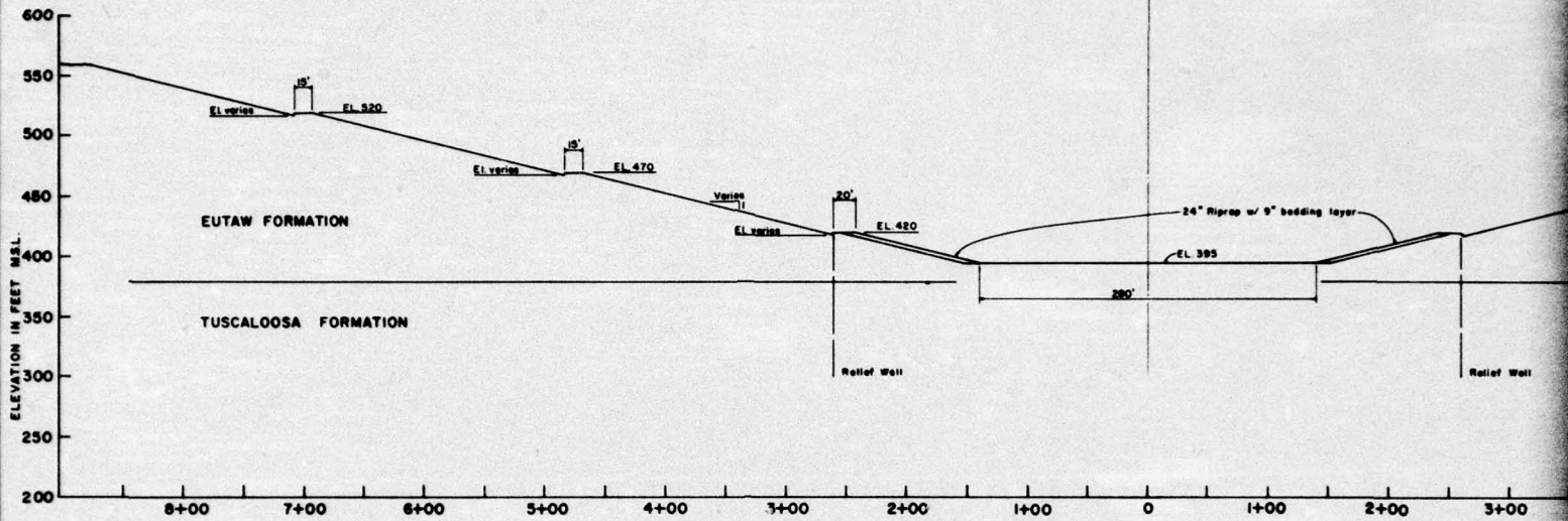
TYPICAL SECTION BETWEEN STA. 12,120+00 AND STA. 13,150+00
