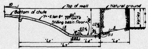
TYPICAL SECTION APRON TYPE
