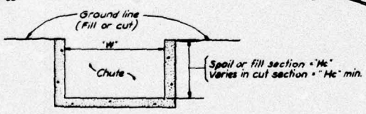
SECTION C-C
