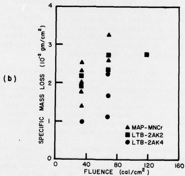
Figure 4. Fused-silica substrate; fluence incident on 30-mil ( 7.62 \times 10^{-2} -cm) carbon filter: (a) impulse versus fluence and (b) specific mass loss versus fluence.
