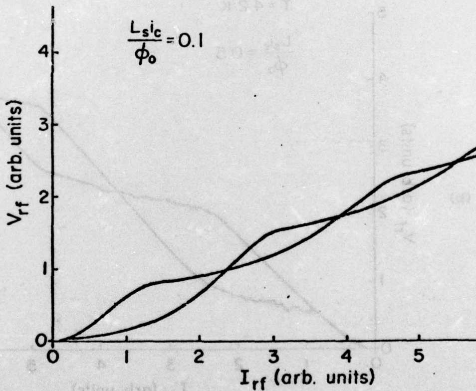
FIGURE 11. Simulated rf I-V characteristics for the low critical current SQUID. In the simulations \omega L_S R_S = 0.1 , K^2 Q = 4 . The tuning is close to optimum.
