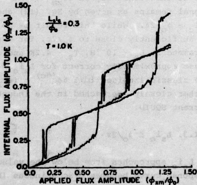
FIGURE 8. \phi_m - \phi_{xm} rf response curve calculated numerically from a noise term included for various values of L_s/C . Again the drive frequency \omega = 0.1R_s/L_s . For clarity only the curve for \phi_x^{(dc)} = n\phi_0 is shown in (a). The simulation assumes T_s = 1K and L_s = 10^{-9}H .
