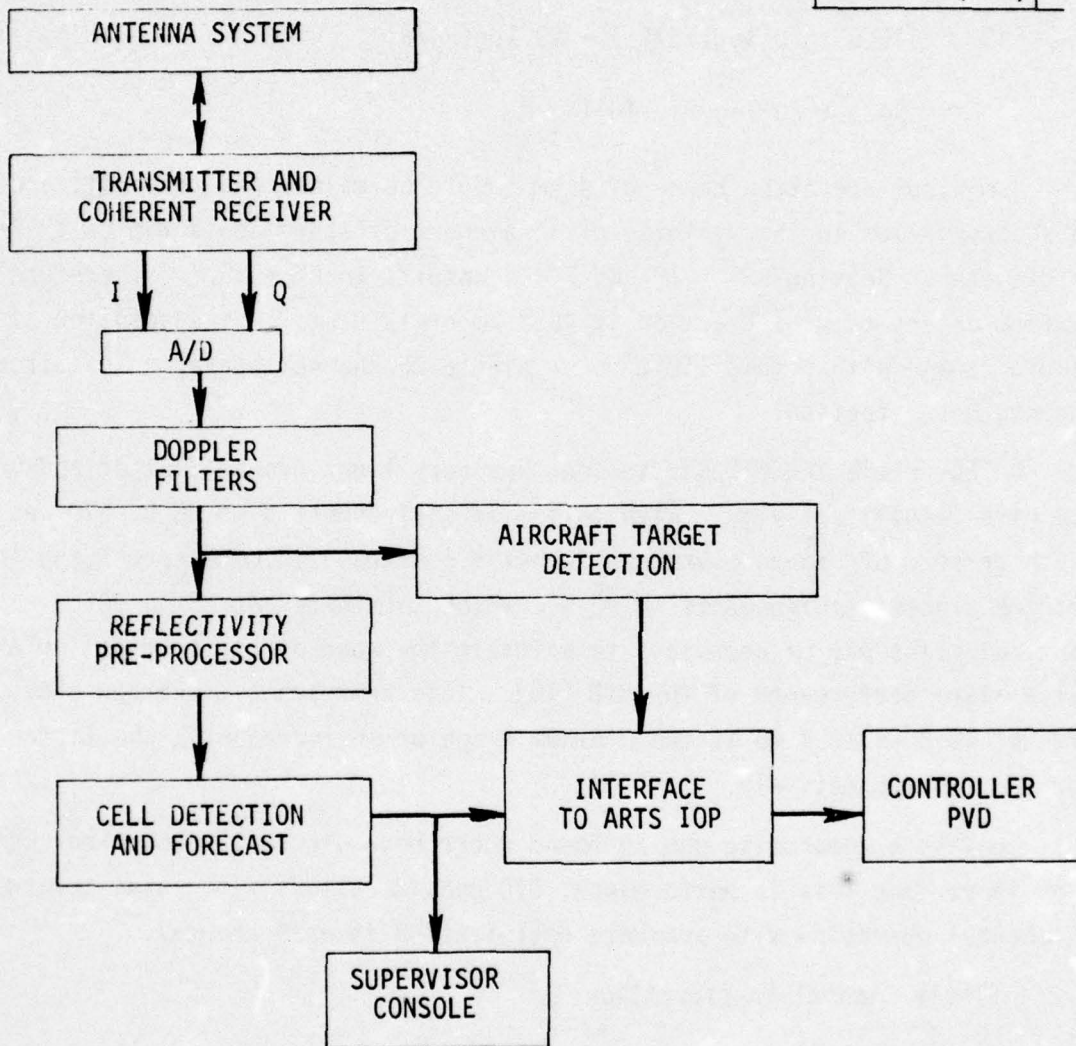
Fig. 3.1 Single RF channel configuration.
