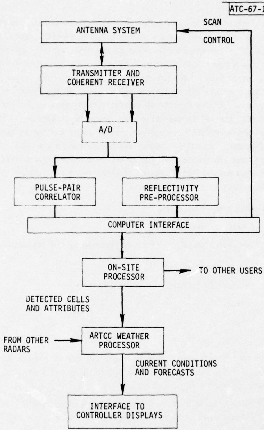
Fig. 5.1 Weather radar for ATC and other users.
