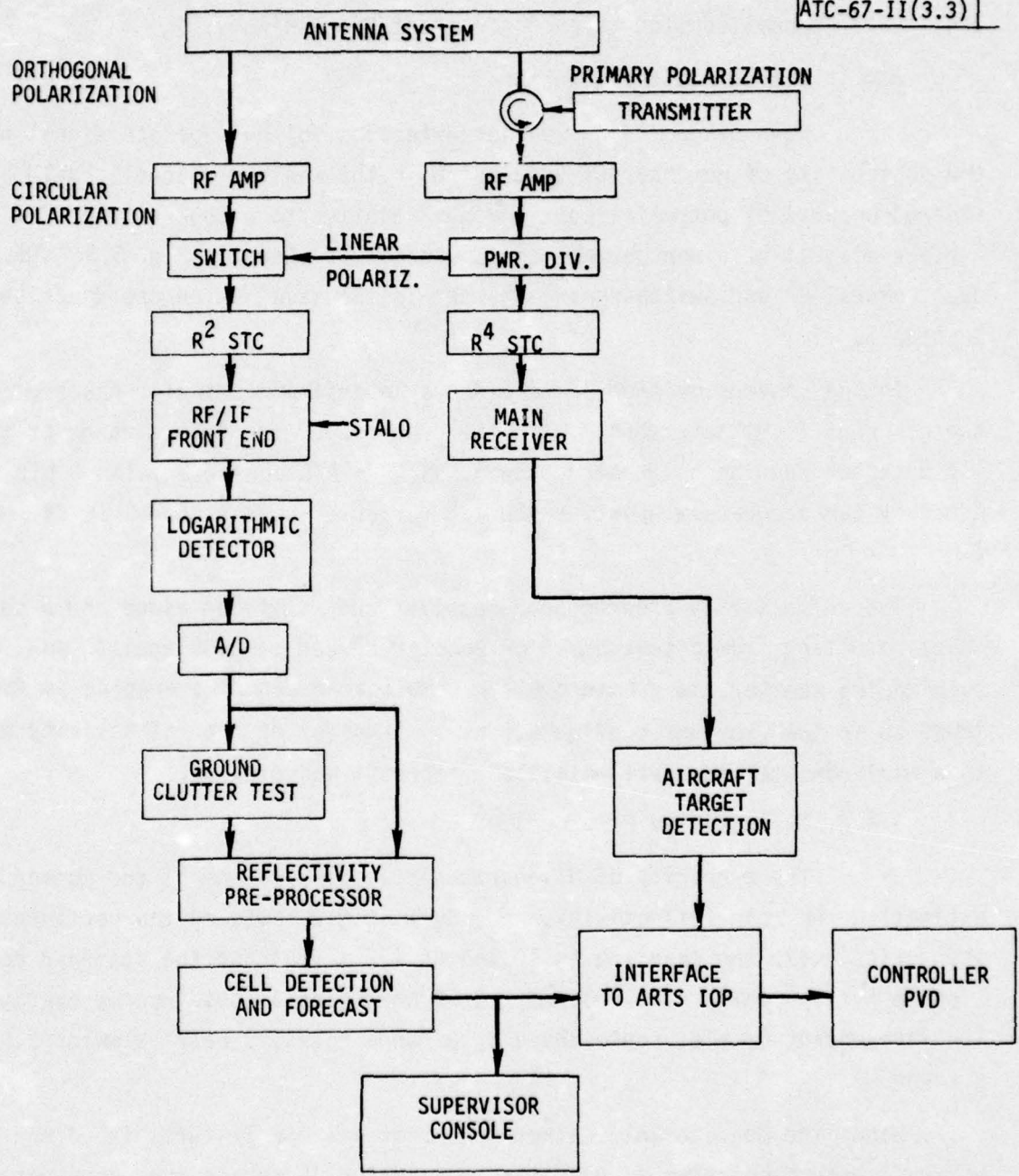
Fig. 3.3 Dual RF channel configuration noncoherent processor.
