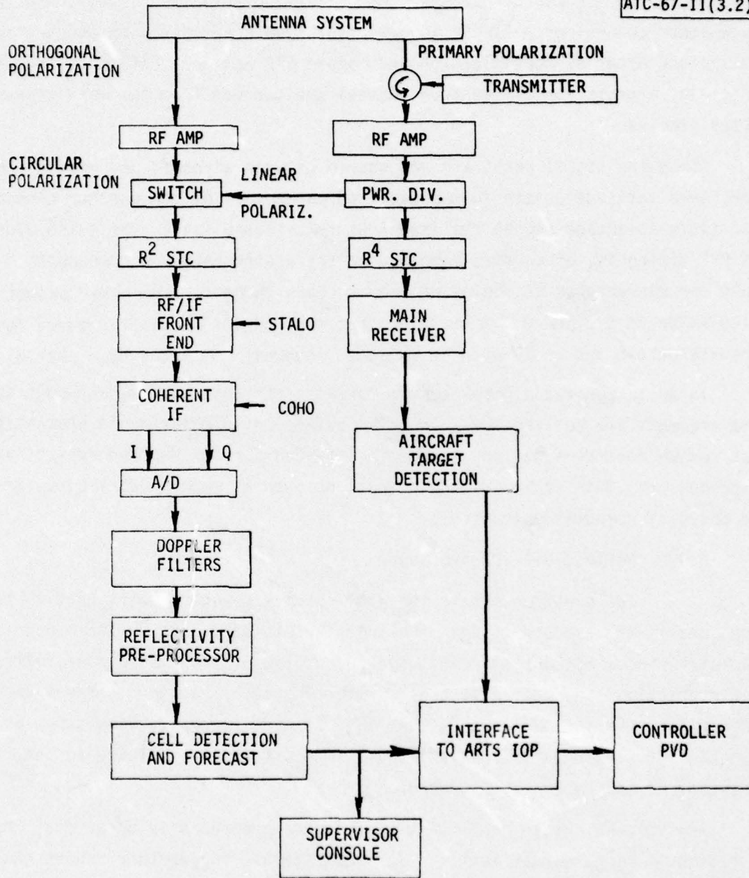
Fig. 3.2 Dual RF channel configuration coherent processing.
