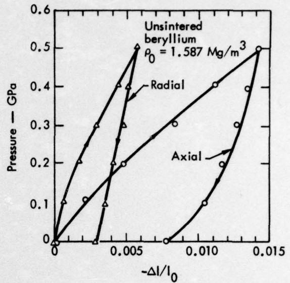
Fig. 9. Strain in radial and axial directions as a function of hydrostatic pressure for unsintered beryllium.
