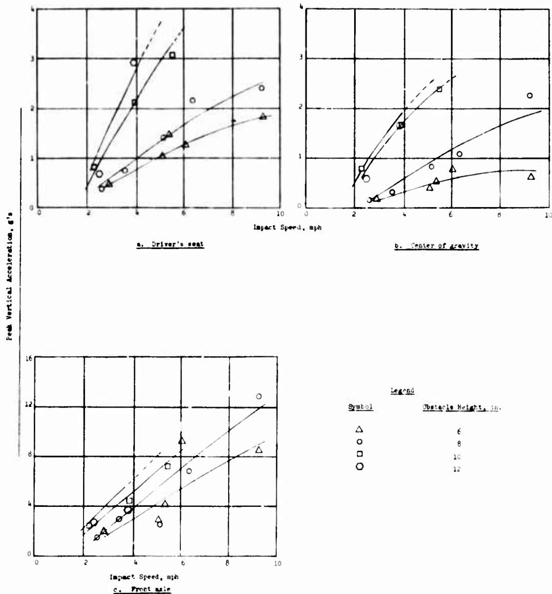
PEAK VERTICAL ACCELERATION-IMPACT SPEED RELATIONS FOR SELECTED OBSTACLE HEIGHTS AND VEHICLE POSITIONS (XM410E1, MEASURED DATA, 20-PSI TIRE PRESSURE)
