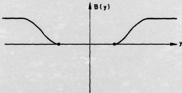
Fig. 9 - Solution with electron pressure included
