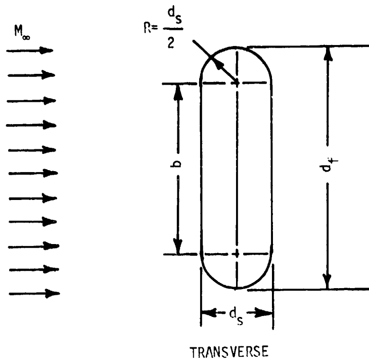
Fig. B-1 Aligned and Transverse Orientation of A Rectangular Injector With Rounded Ends
