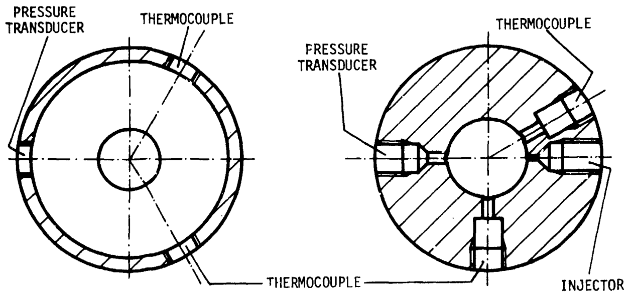
Figure 2: Test Nozzle
