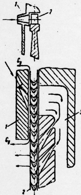
Fig. 2. Pressure stage with re-supply (steam supply from two sides). 1 - nozzle; 2 - moving blades; 3 - rotating chamber.
