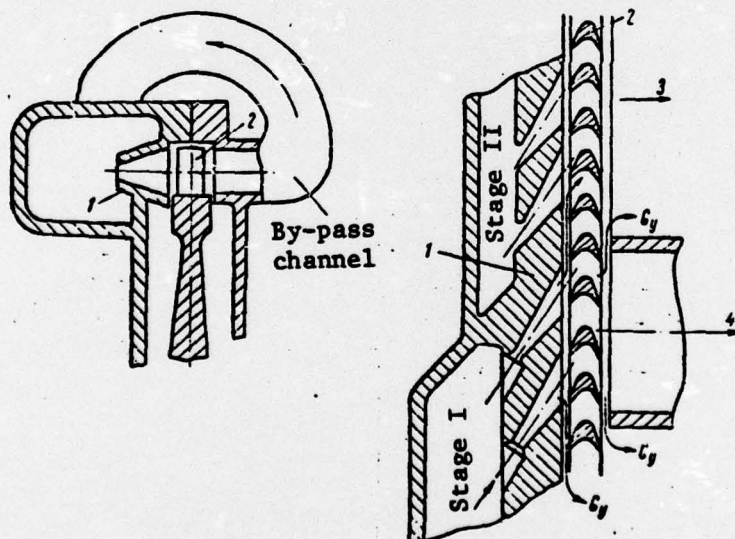
Fig. 3. Pressure Stage with Re-Supply (Steam Supply from One Side). 1 - nozzle; 2 - moving blades; 3 - outlet from stage II; 4 - entrance to stage II through by-pass channel.
