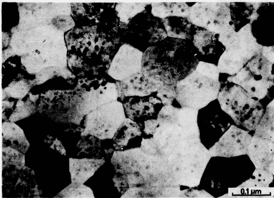
Figure 6. - Dispersion of fine TiNi_3 particles in a "ARE" Ti-10 % Ni-C coating, deposited at 700°C.
