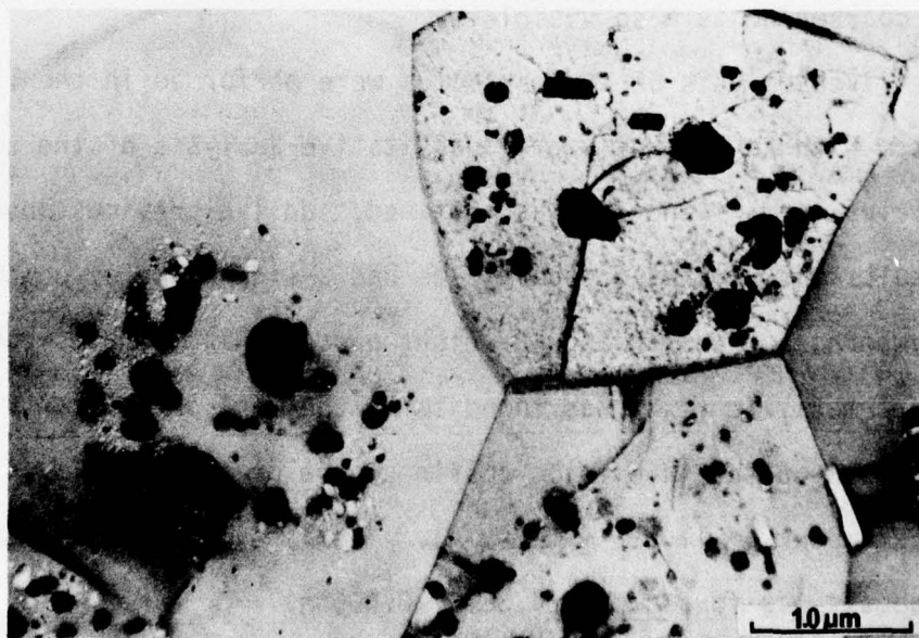
Figure 3 - The presence of dislocations inside TiC grains around Ti_xNi_y particles. (Ti-10 % Ni-C coating deposited at a 1000°C).
