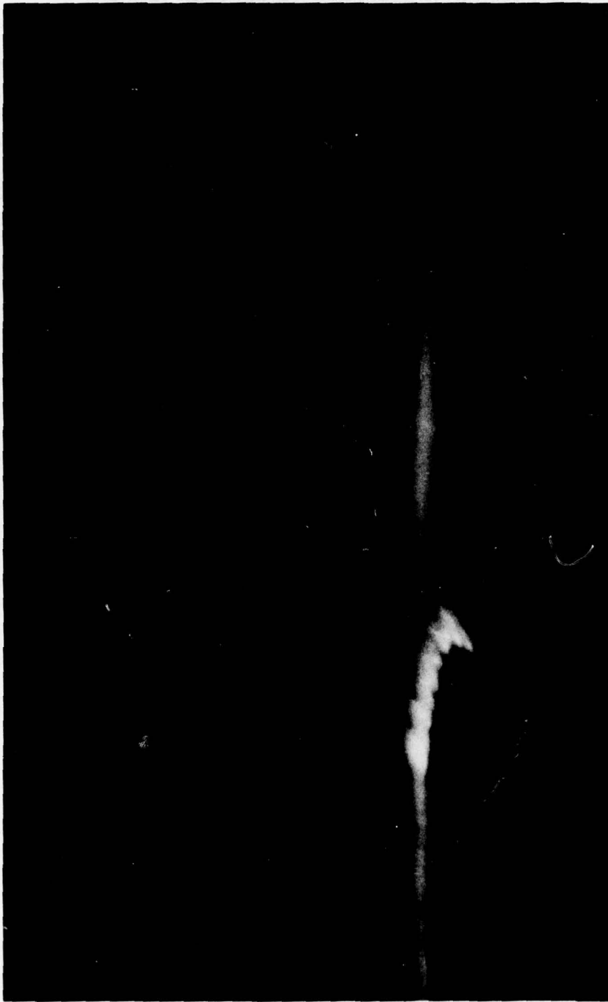
Fig. 6 — Sept. 11, 1973, at 2152 UT, from 48^{\circ}.6S - 68^{\circ}.8E . Auroral horizon midpoint at 71^{\circ}.5S - 95^{\circ} , 0029 hrs LGMT. An intense green rayed arc that folds back upon itself and blends in with a less bright homogeneous band extending toward the horizon as a thin layer. Antares, \alpha Scorpii, is the bright star at the right. Frame 3135.
