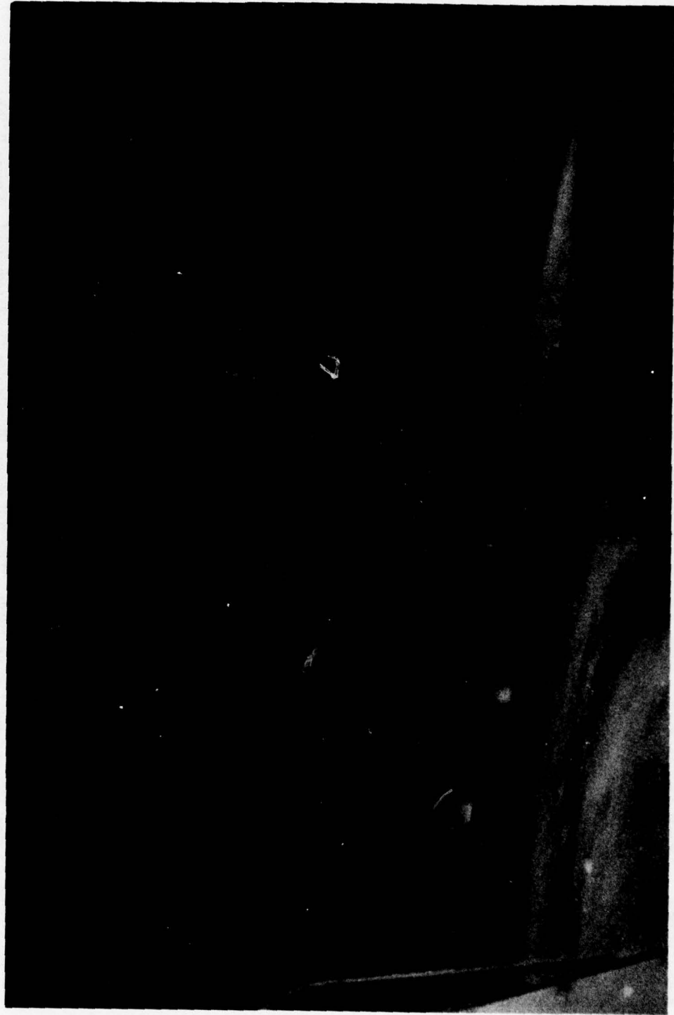
Fig. 3 - Sept. 12, 1973, at 1759 UT, from 42^{\circ} 9S - 101^{\circ} 6E . Auroral horizon midpoint at 70^{\circ} S - 137^{\circ} , 2236 hrs LGMT. Discrete auroral forms along with diffuse bands, two luminous layers and a red auroral glow above. The Earth is illuminated by the full moon and reflected auroral light. The brightest star is \theta Centauri. Frame 3145.
