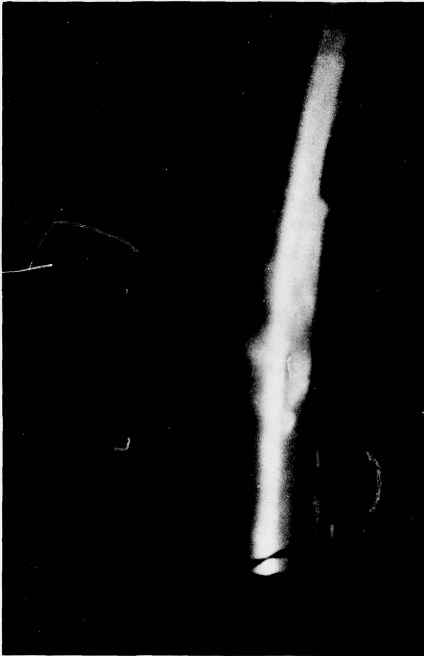
Fig. 2 — Sept. 9, 1973, at 2140 UT from spacecraft position 42^{\circ}48' - 62^{\circ}48'E . Auroral horizon midpoint at 67^{\circ}S - 97^{\circ} , 2322 hrs LGMT. Very intense green emission from the particle-excited atomic oxygen line at 5577 \text{ \AA} extends in a band parallel to the earth horizon, with some discrete auroral forms also present. Emission from atomic oxygen at 6300-6364 \text{ \AA} is also prominent as a red glow extending upward from the green band to beyond 250 km. Rays above the main layer parallel the geomagnetic lines of force. The bright star near mid-photo is \theta Centauri. The structure at left is part of an ATM solar panel with its antisolar side illuminated by the full moon. Frame 3107.
