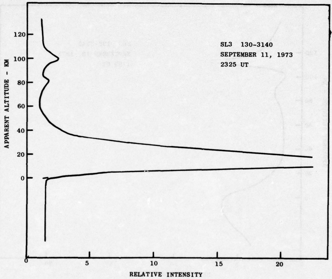
Fig. 9 - Apparent altitudes of luminous layers in Fig. 7
