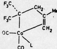
(III, L = CO) (VII, L = PPh 3 ) (VIII, L = AsPh 3 )
