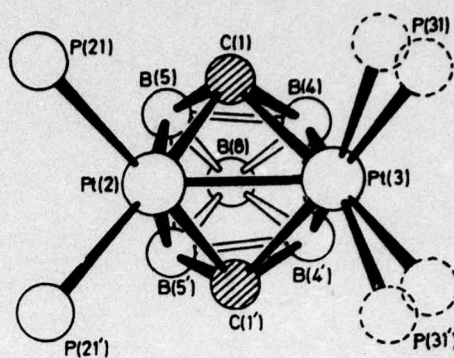
Molecular structure of closo-2,3-[(Et 3 P) 2 ] 2 -1,2,3,6-CPt 2 CB 8 H 7 . Phosphinoethyl groups are omitted for clarity.
