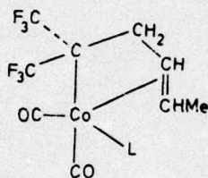
(IV a, L = CO) (IX, L = PPh 3 ) (X, L = AsPh 3 )
