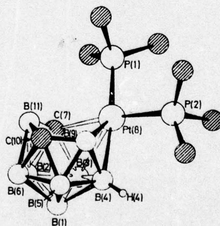
Molecular structure of nido-8,8-[(Me 3 P) 2 ]-7,8,10-CPtCB 8 H 10 .
