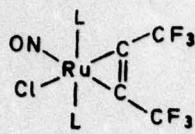
(II) L = PPh 3 (VI) L = PMePh 2 (IX) L = PMe 2 Ph
