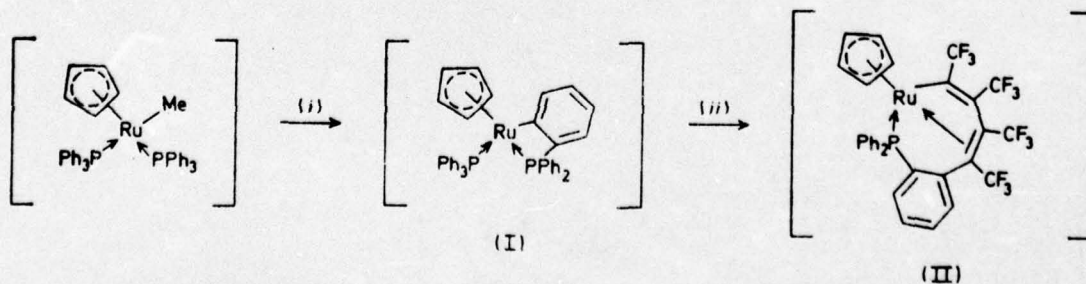
Scheme 4. (i). Refluxing decalin, -CH_3 ; (ii). C_2(CF_3)_2
