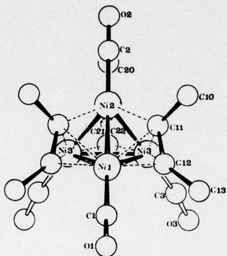
Molecular structure of [\text{Ni}_4(\text{CO})_4(\text{CF}_3\text{C}_2\text{CF}_3)_3] . Fluorine atoms omitted for clarity. The Ni-CO bond distances average 1.81 (6) Å and the three Ni(apex)-Ni(basal)-CO fractions are each nearly linear. The three OC-Ni(apex)-Ni(basal) are each nonlinear with the OC-Ni(apex) vector nearly collinear with the idealized C_3 axis of the molecule.
