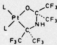
(Ia) L = PPh 3 (IIIa) L = PMePh 2
