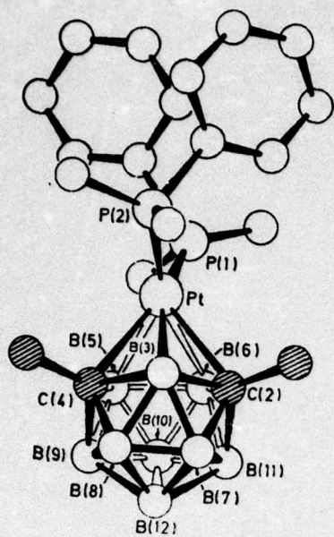
General view of the molecule 1,1-(PhMe 2 P) 2 -2,4-Me 2 -1,2,4-PtC 2 B 8 H 8
