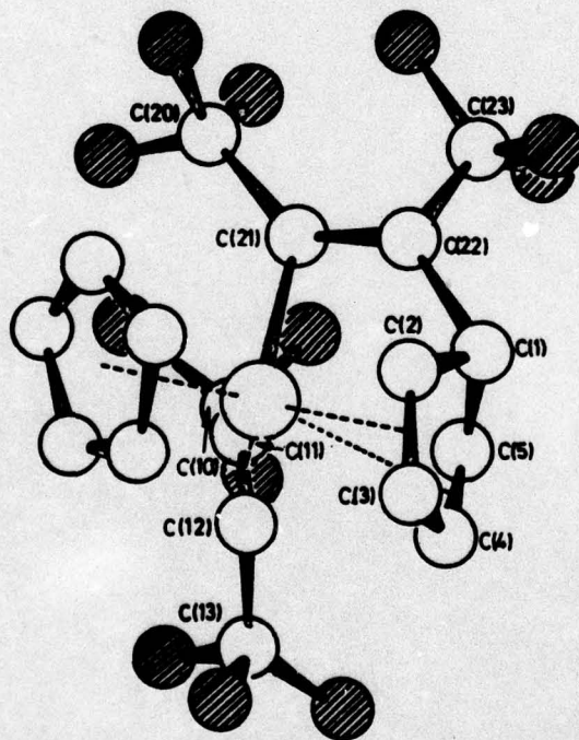
Molecular structure of [Mo(CF_3)_2(CF_3C_6H_5)]
