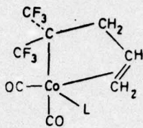
(II, L = CO) (V, L = PPh 3 ) (VI, L = AsPh 3 )
