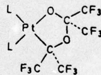
(II) L = PMePh 2 (V) L 2 = Ph 2 PCH 2 CH 2 PPh 2 (IX) L = P(OMe) 3 (XI) L 2 = 1,5-C 6 H 12
