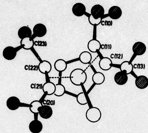
Molecular structure of [W(Cl)(CF_3C_6CF_3)(\eta^5-C_6H_5)] .
