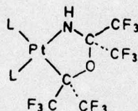
(Ib) L = PPh 3 (IIIb) L = PMePh 2
