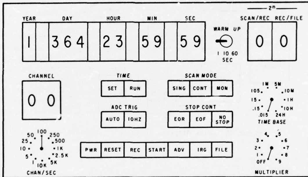
Figure 21. Data logger with enlargement of control and monitoring panel.
