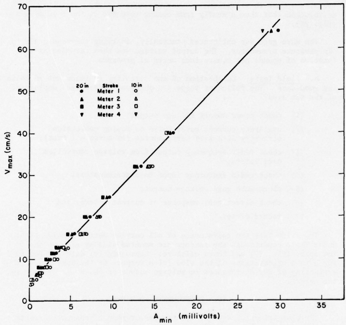
Figure 24. B-7 sensor, V_{max} versus A_{min} .
