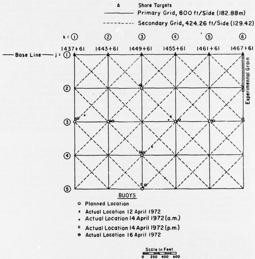
Figure 35. Buoy shore-marker grid.
