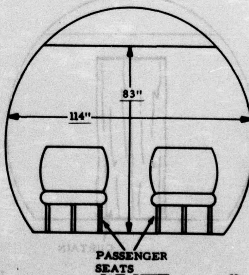
FIGURE 5B. PARTITION AND CURTAIN CONFIGURATIONS (SHEET 2 OF 4)
