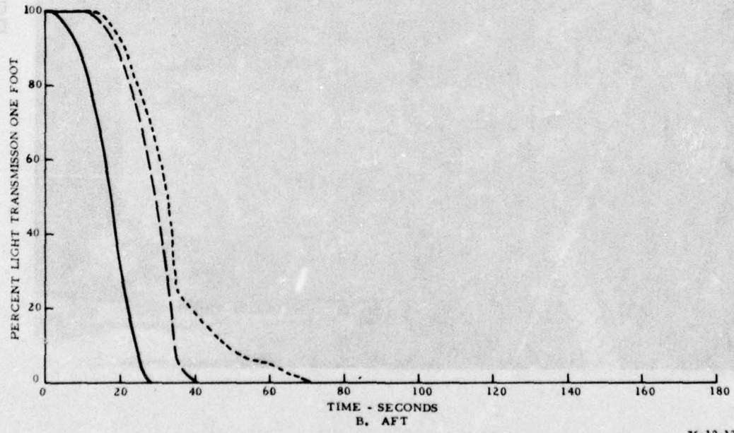
FIGURE 10. LARGE-FIRE SMOKE LEVELS (FIVE FOAM PANELS)
