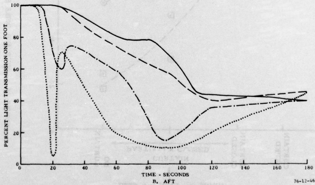
FIGURE 43. SMOKE LEVELS USING DECORATIVE-TYPE PARTITION (2,800 ft 3 /min AIRFLOW)
