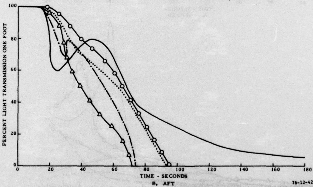
FIGURE 39. SMOKE LEVELS USING DECORATIVE-TYPE PARTITION (NO AIRFLOW)
