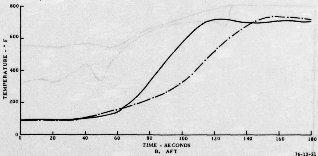
FIGURE 18. TEMPERATURE LEVELS (AIRFLOW THROUGH DOOR EXIT)
