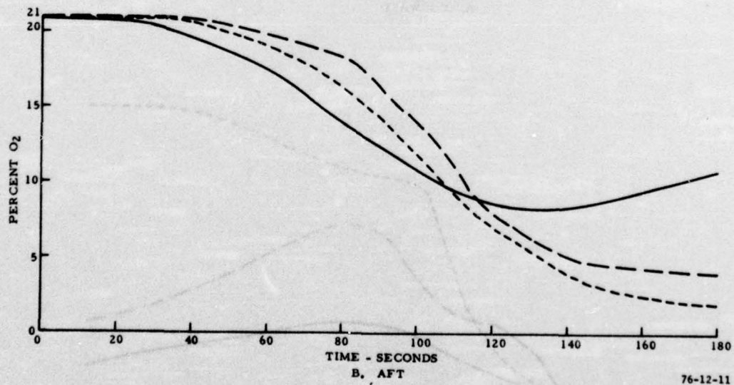
FIGURE 8. LARGE-FIRE OXYGEN LEVELS (FIVE FOAM PANELS)
