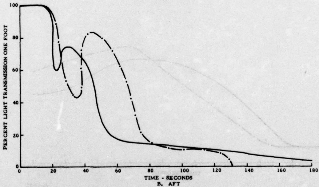
FIGURE 25. SMOKE LEVELS USING FAR PARTITION (2,800 ft 3 /min AIRFLOW)
