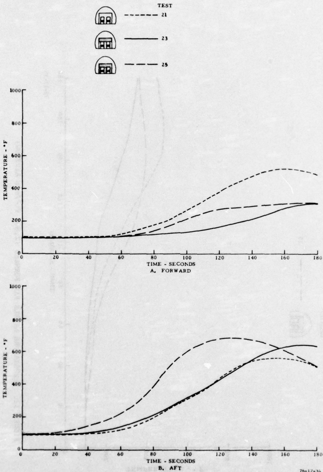
FIGURE 31. TEMPERATURE LEVELS WITH SEATS INSTALLED AT PARTITION (2,800 ft 3 /min AIRFLOW)
