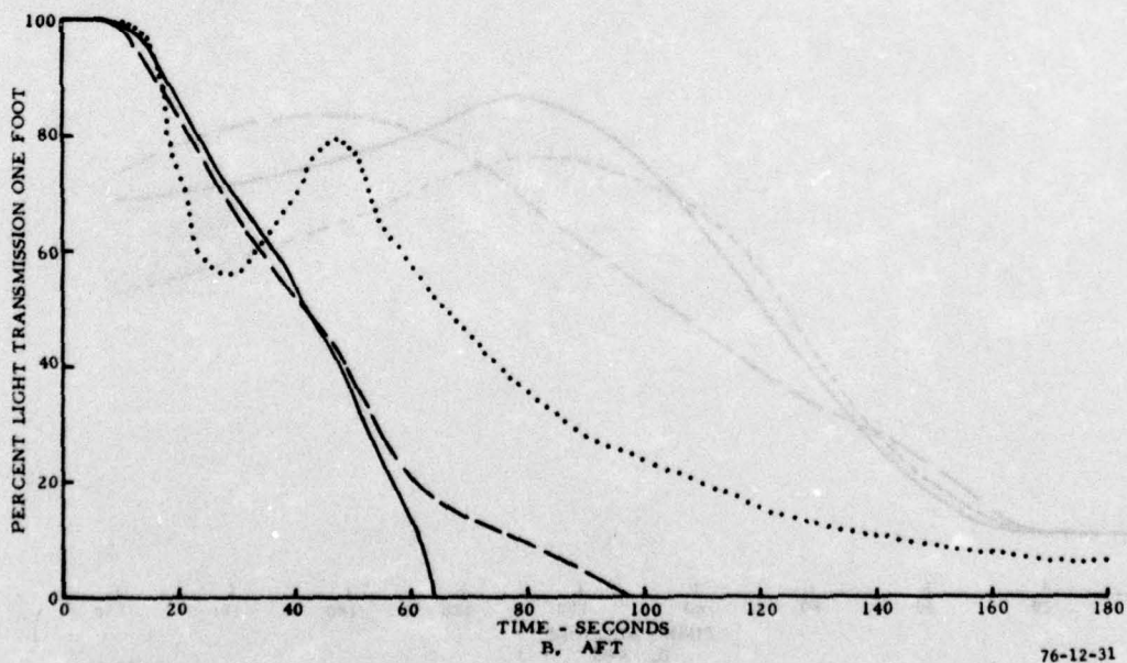
FIGURE 28. SMOKE LEVELS WITH SEATS INSTALLED AT PARTITION
