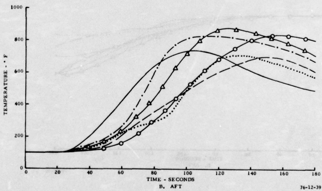
FIGURE 36. TEMPERATURE LEVELS USING DECORATIVE PARTITION (NO AIRFLOW)
