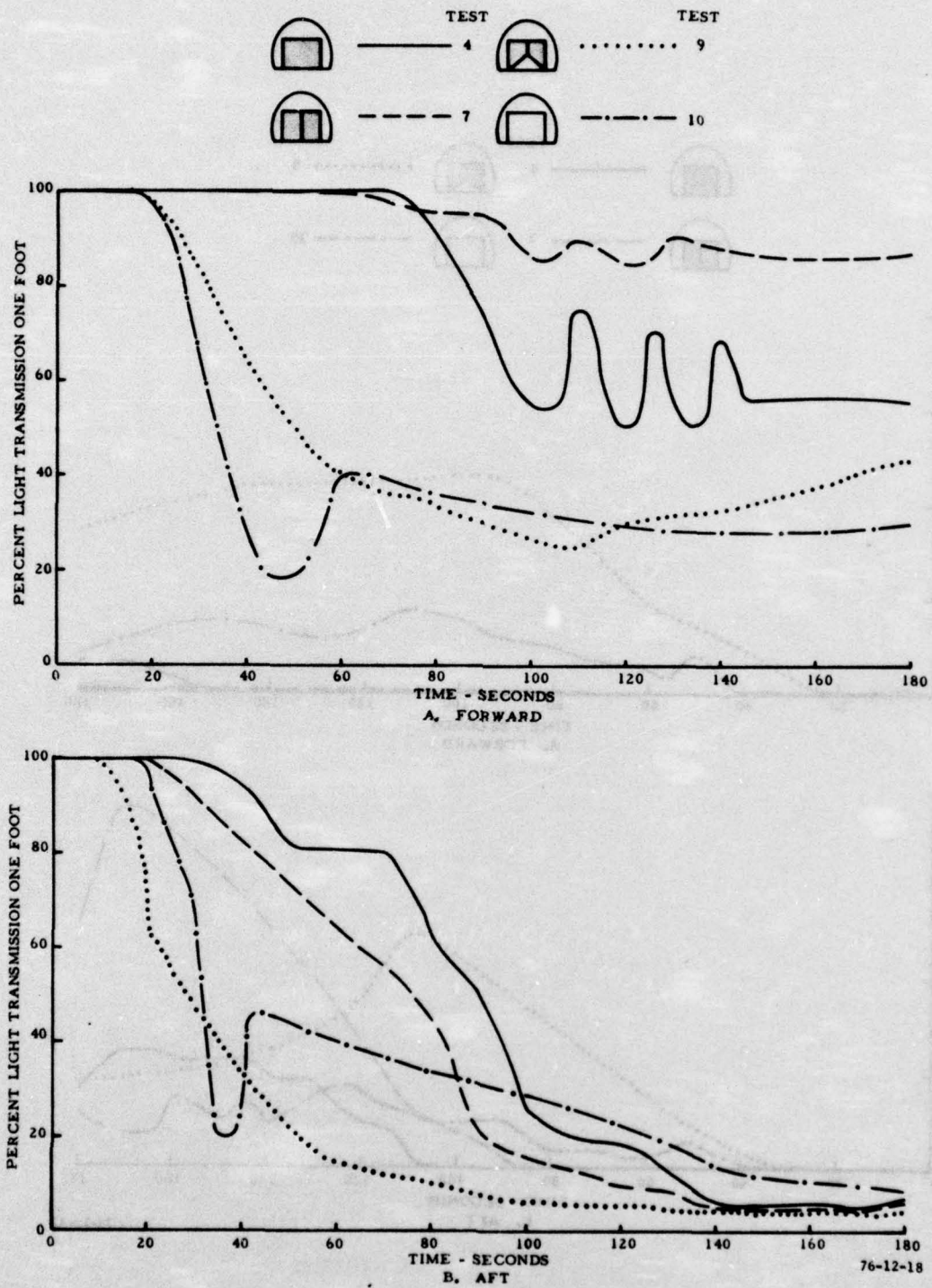
FIGURE 15. SMOKE LEVELS USING TWO FOAM PANELS (NO AIRFLOW)
