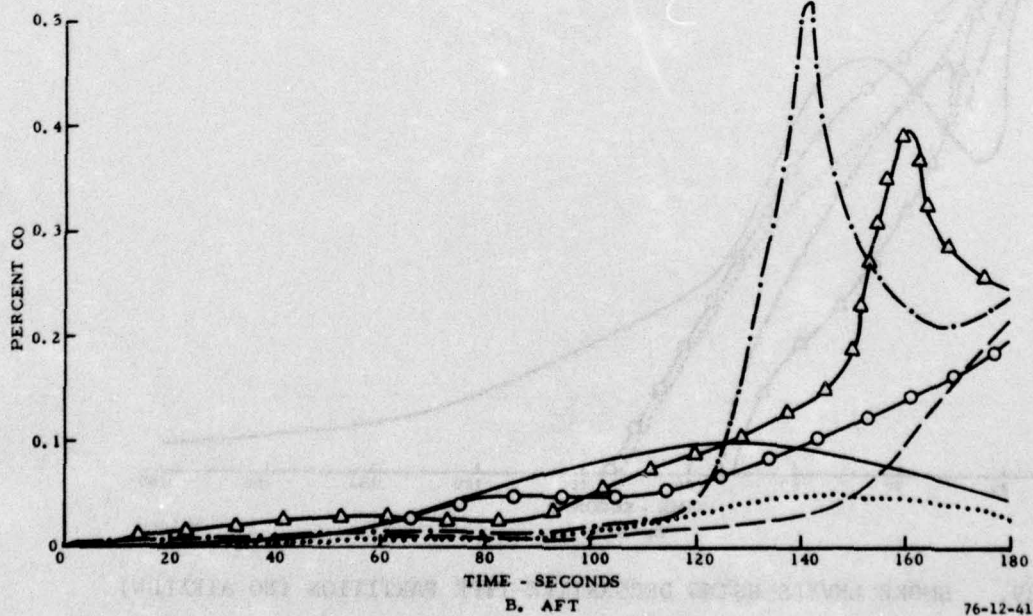
FIGURE 38. CO LEVELS USING DECORATIVE-TYPE PARTITION (NO AIRFLOW)
