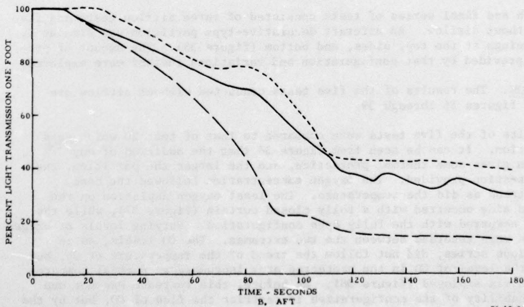
FIGURE 33. SMOKE LEVELS WITH SEATS INSTALLED AT PARTITION (2,800 ft 3 /min AIRFLOW)
