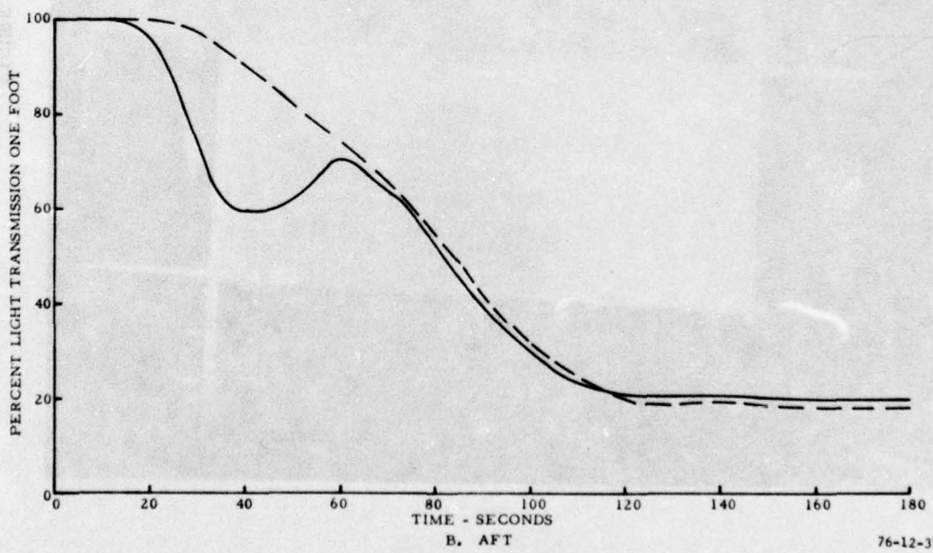
FIGURE 34. SMOKE LEVELS USING 18-INCH HEADER
