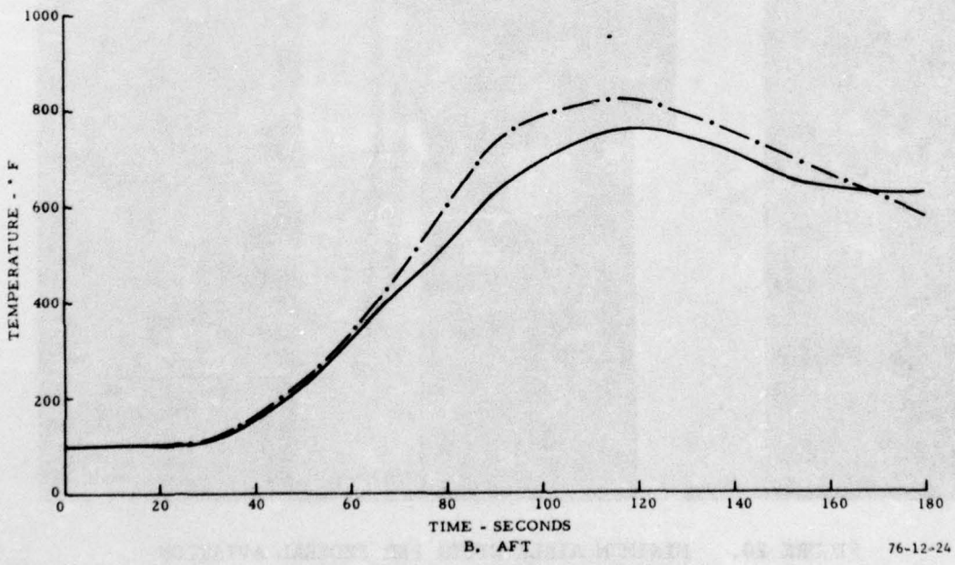
FIGURE 21. TEMPERATURE LEVELS USING FAR PARTITION (NO AIRFLOW)
