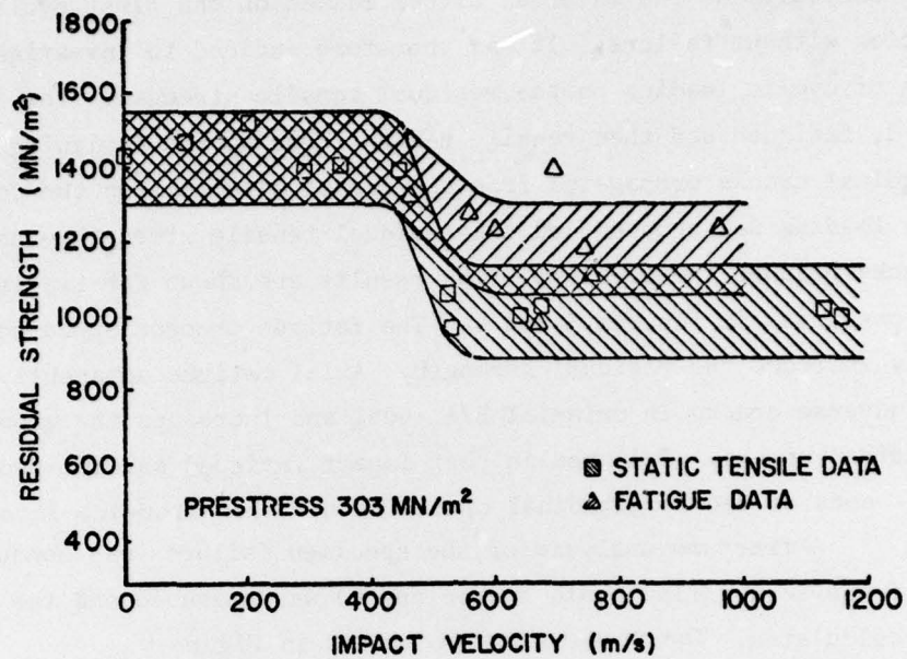
Figure 4. Residual Strength of B-6061 Al Versus Impact Velocity Based on Uncracked Area, Tensile and Fatigue Data, Prestress 303 \text{ MN/m}^2 Thickness 1.35 \text{ mm} . (From Jacques 2 )
