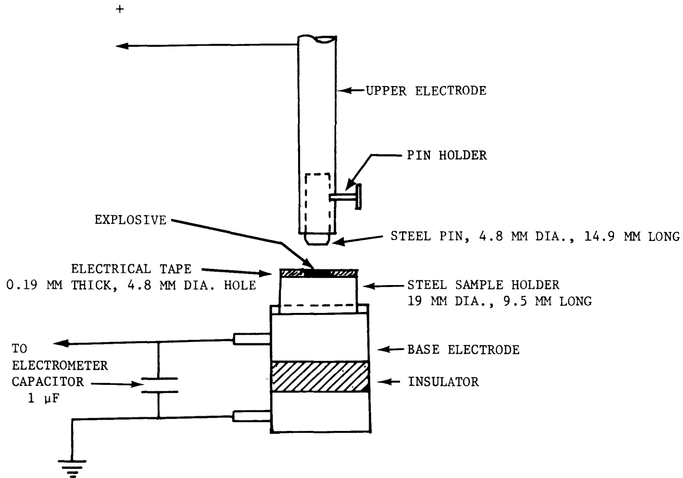
Fig 7 Plane-to-plane electrode assembly
