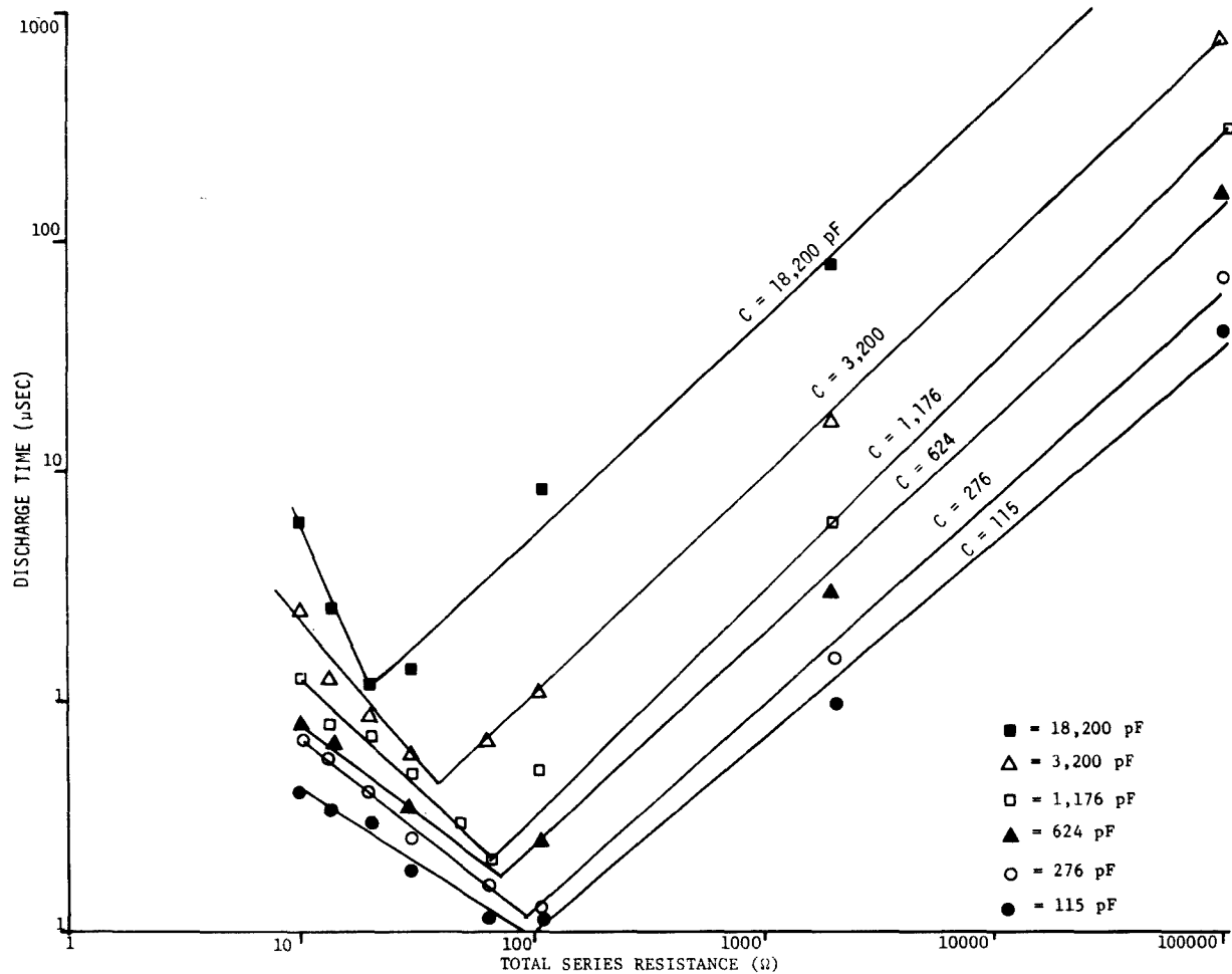
Fig 2 Dependence of duration of discharge on series resistance and charging capacitance (Series resistance includes the 7.5 ohm resistance of the gap. Minimum discharge time occurred when the discharge circuit became critically damped.)
