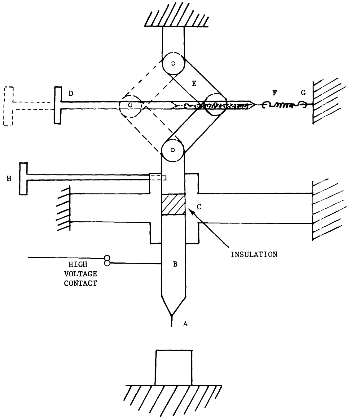
Fig 9 Schematic showing operation of approaching assembly
