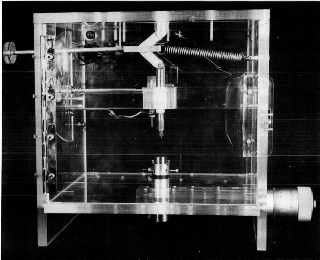
Fig 5 Approaching-electrode assembly
