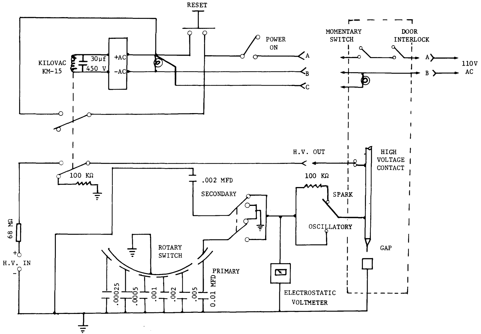
Fig 10 Proposed electrical circuit
