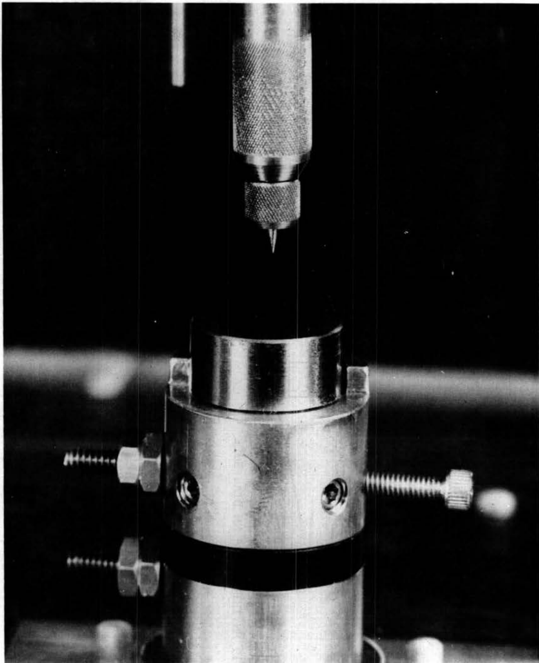
Fig 6 Needle-plane electrode assembly
