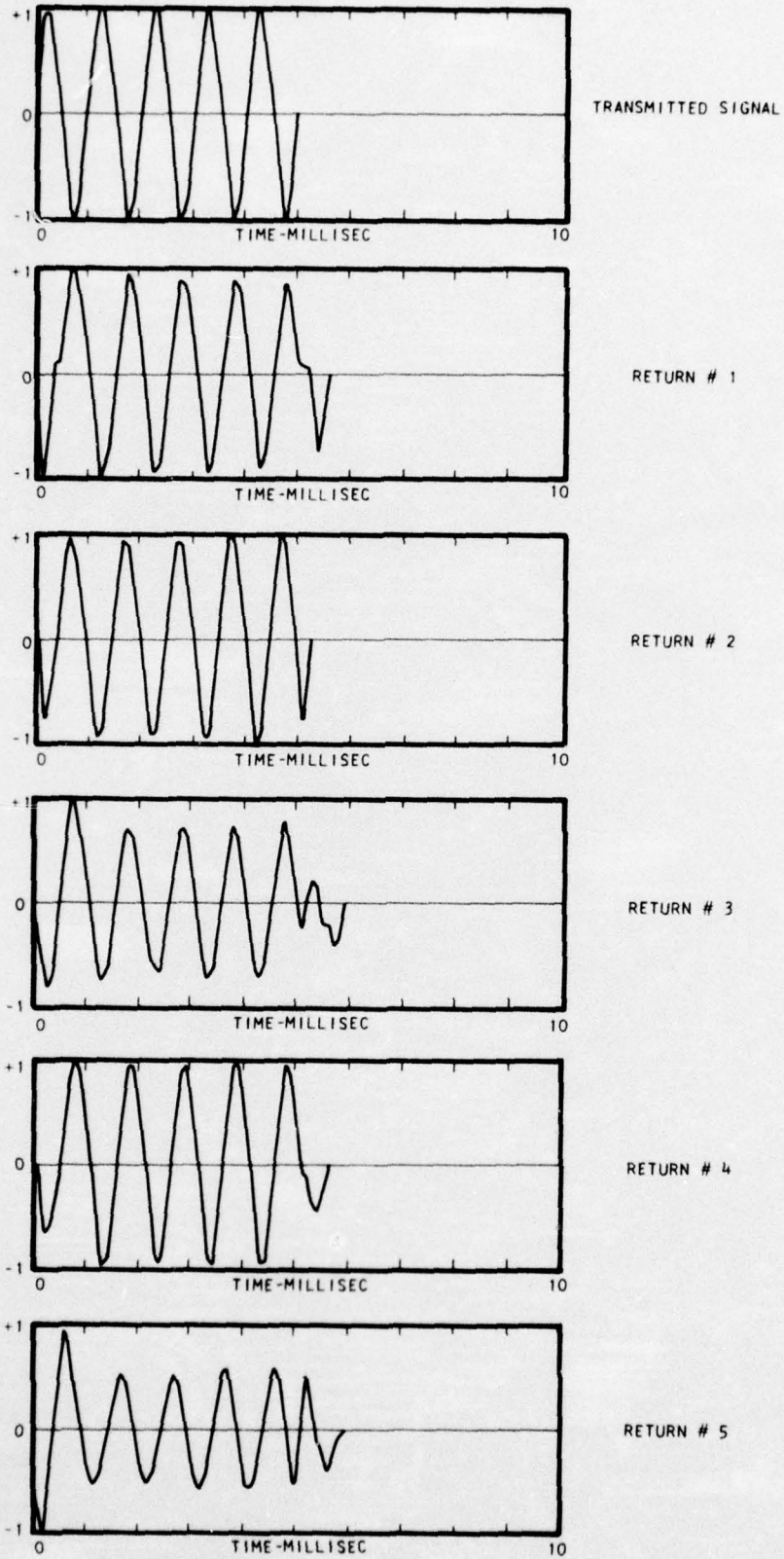
FIG. 5-3 - TRANSMITTED SIGNAL AND FIVE RETURNS FOR A 20 KNOT WIND GENERATED SURFACE
