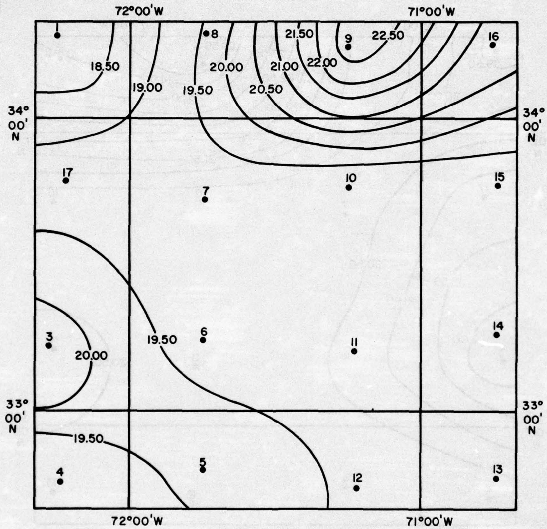
FIGURE 6c AREAL DISTRIBUTION OF TEMPERATURE AT 100 METERS
