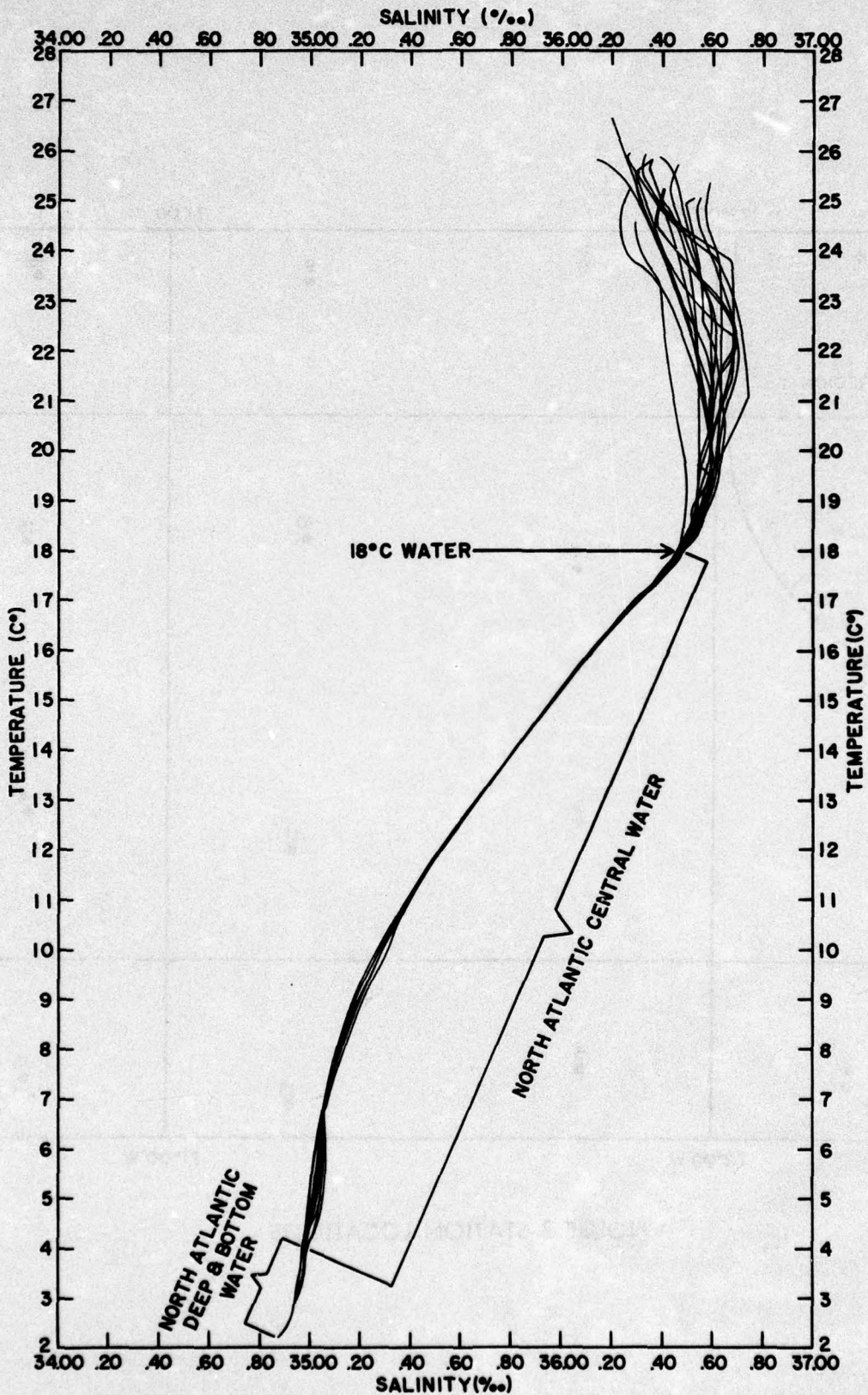
FIGURE 3 COMPOSITE OF TEMPERATURE-SALINITY
