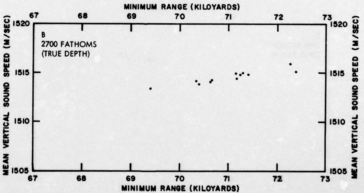
FIGURE 13b MEAN VERTICAL SOUND SPEED VS. MINIMUM RANGE TO CONVERGENCE ZONE
