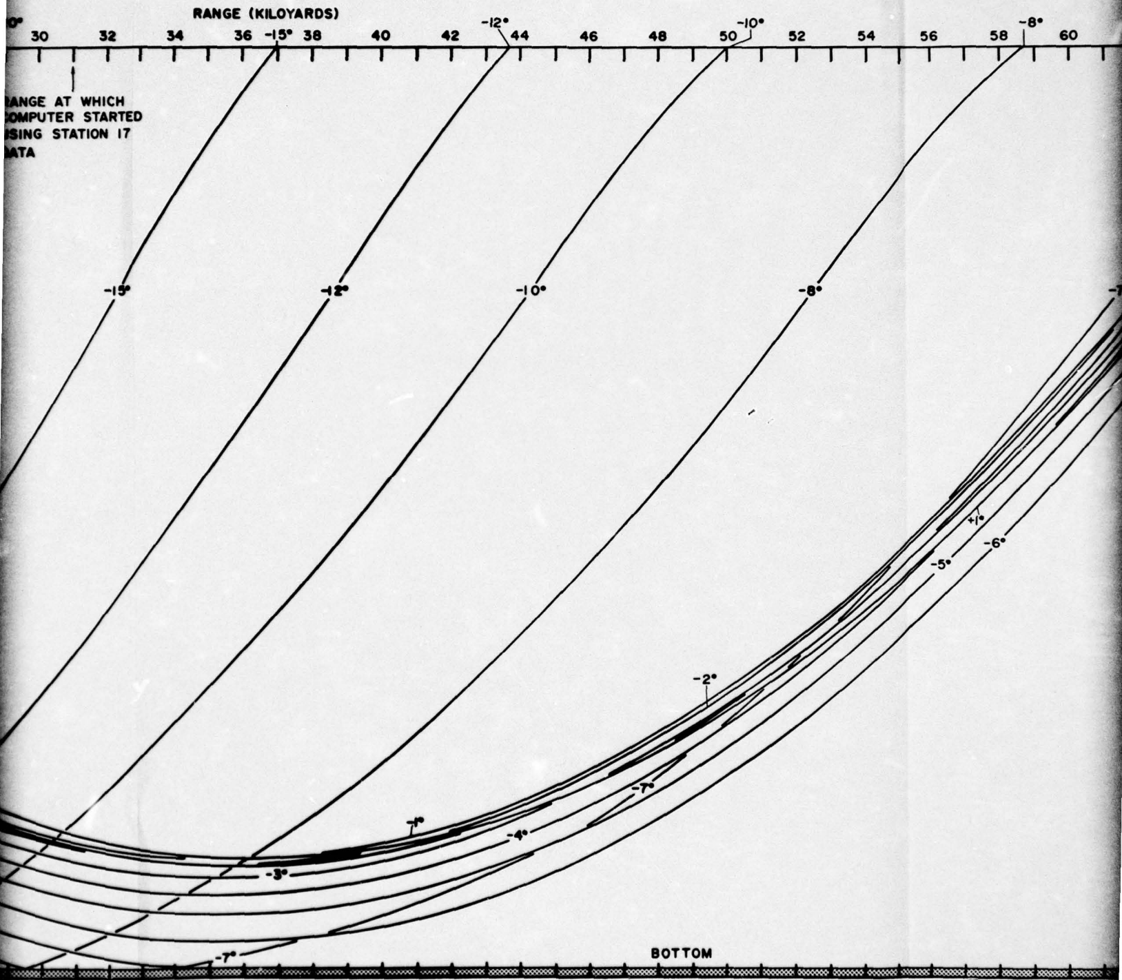
DIAGRAM INCORPORATING HORIZONTAL CHANGES
