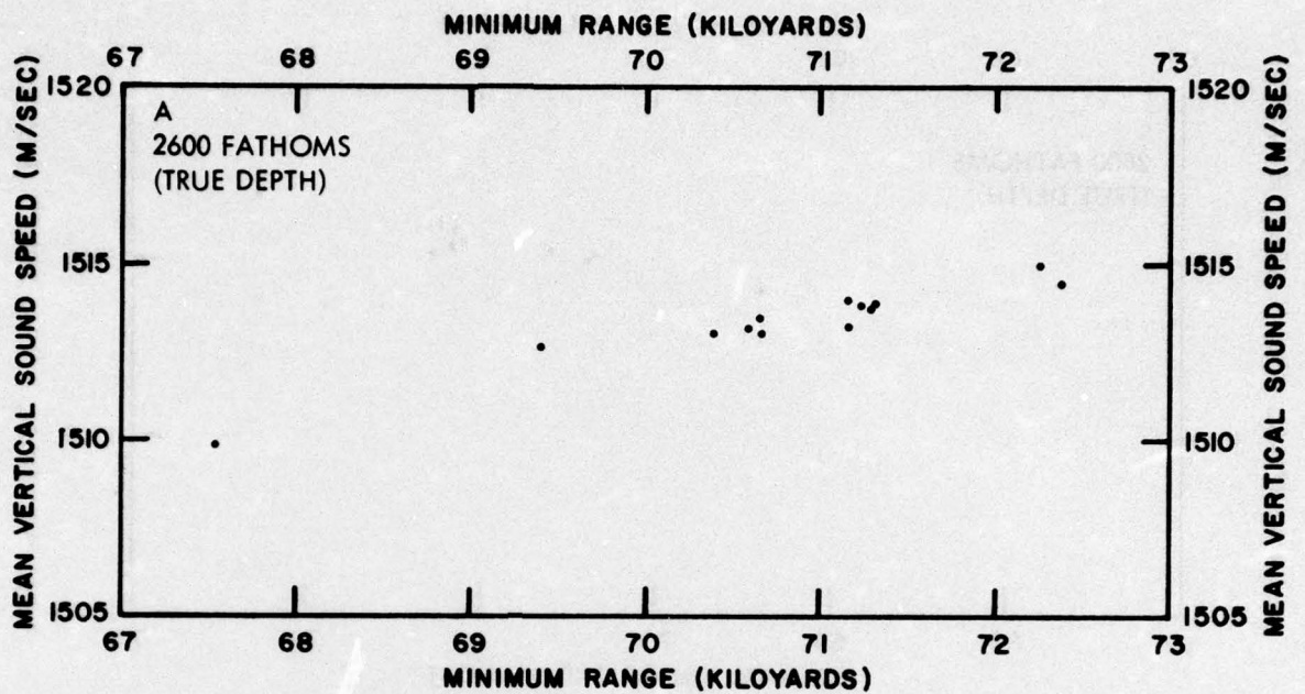
FIGURE 13a MEAN VERTICAL SOUND SPEED VS. MINIMUM RANGE TO CONVERGENCE ZONE
