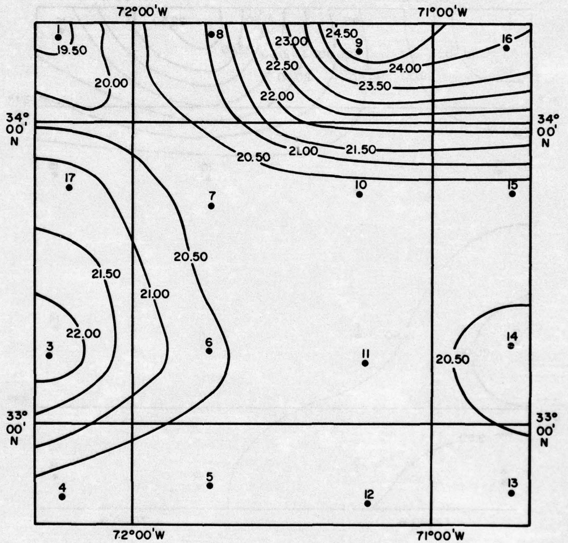
FIGURE 6b AREAL DISTRIBUTION OF TEMPERATURE AT 50 METERS
