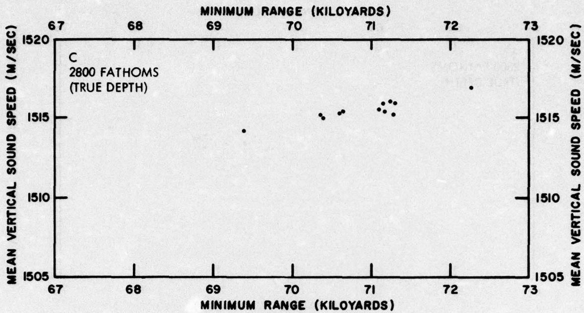
FIGURE 13c MEAN VERTICAL SOUND SPEED VS. MINIMUM RANGE TO CONVERGENCE ZONE
