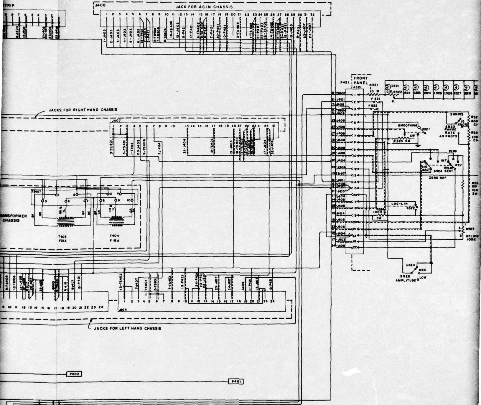
SONAR SIGNAL ANALYZER FRAME AND INTERCONNECTIONS FIGURE C-19
