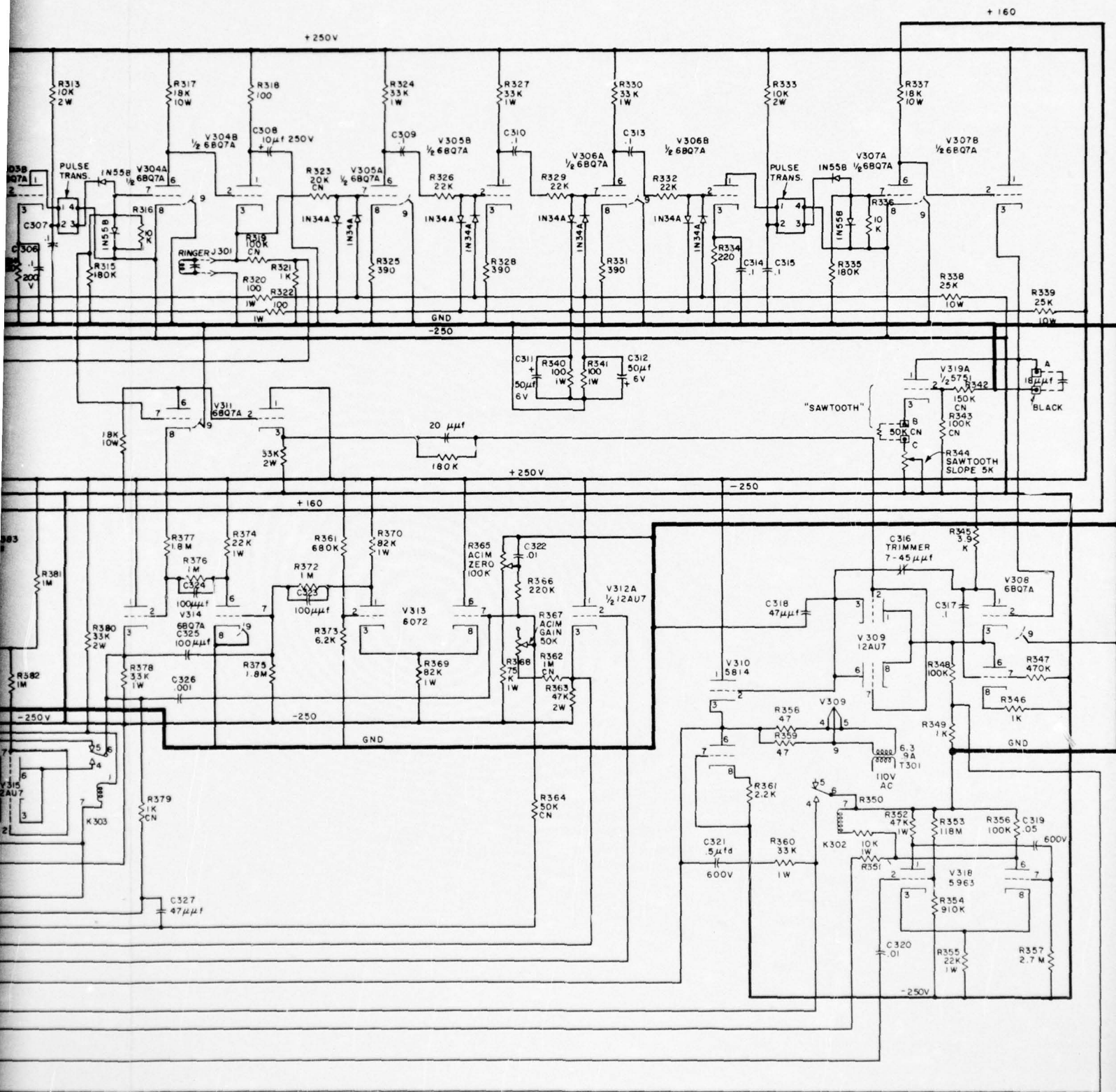
SONAR SIGNAL ANALYZER ACIM CHASSIS FIGURE C-18
