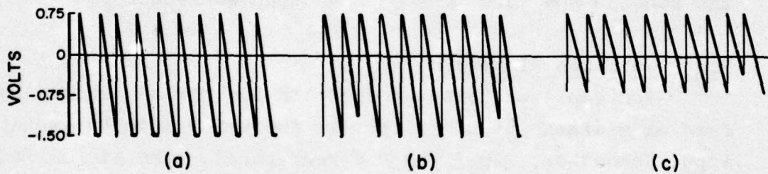
Figure 5-2. Wave form at the Sawtooth test point (terminal 14, TS-401) when: a) R or C is too small, b) R and C are correct, c) R or C is too large.
