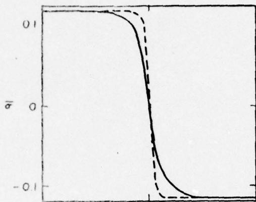
(a) R=3.5, J=0.4
