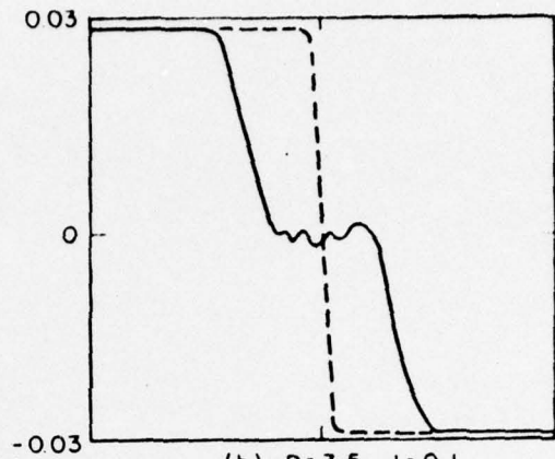
(b) R=3.5, J=0.1
