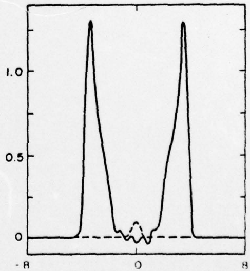
(f) R=3.5, J=0.1
