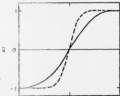
(c) R=3.5, J=0.4
