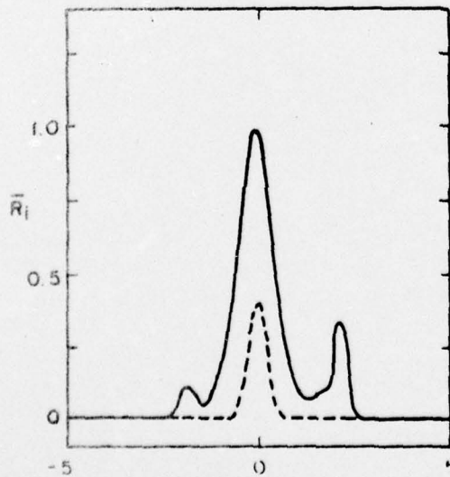
(e) R=3.5, J=0.4
